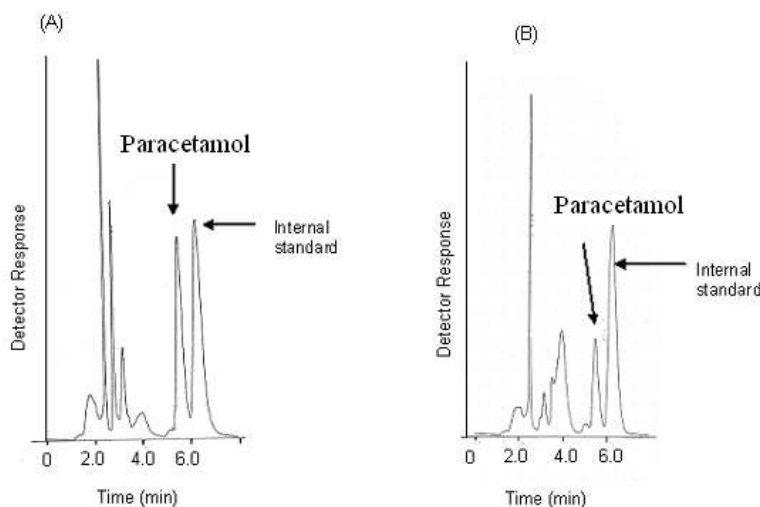
Figure 1: HPLC chromatograms of paracetamol (5.53 min) and the internal standard \beta Hydroxyethyltheophylline (6.46 min) in plasma (A) and urine (B). The peaks were identified by the retention times. The other peaks observed in the chromatograms were attributed to the substances present in matrices.
