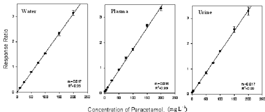
Figure 2: Linearity of the standard curve of paracetamol in water, plasma and urine over concentration range of 0.25-200 mg L -1 . R 2 exceeds 0.99. (Response ratio - Area under curve of paracetamol / Area under curve of internal Standard)
