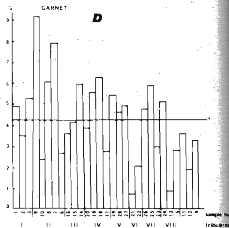
Figures 4a-d — Histograms showing the heavy mineral contents of the samples analyzed.
