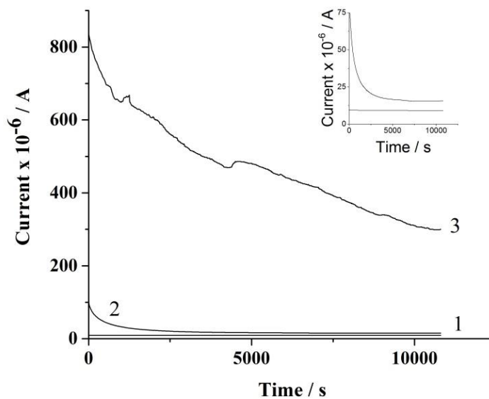
Figure 2 : Discharge characteristics of the cell, Zn / GPE / graphite electrode under different constant loads (1 - 100 kΩ, 2 – 10 kΩ, 3 – 1 kΩ)
