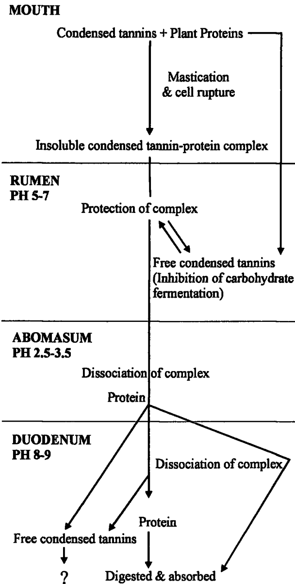
Fig 2. Condensed tannins and protein protection in the rumen (after Mangan, 1990)
