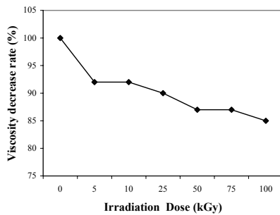
Figure 5: Effect of irradiation on viscosity decrease rate of chitosan solution directly irradiated at doses ranging from 0-100 kGy
