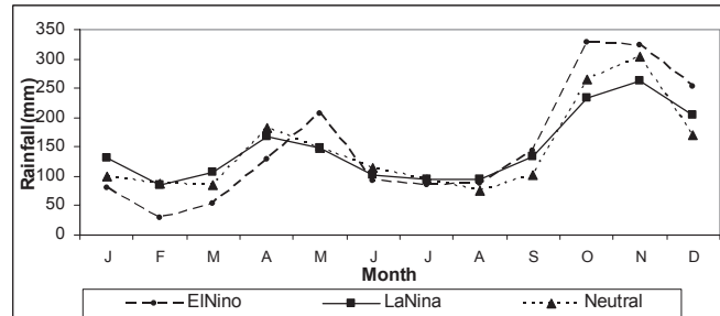
Figure 2: The composite rainfall climatology for all Sri Lanka during El Niño, La Niña and Neutral phases. The characters J to D stand for months from January to December.
