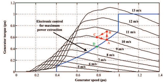
Figure 3: Torque vs. speed characteristics of a variable-speed wind turbine
