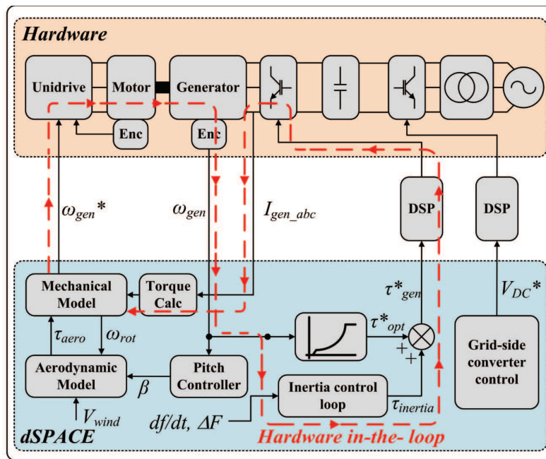
Figure 6: Experiment design block diagram showing the hardware in-the-loop
