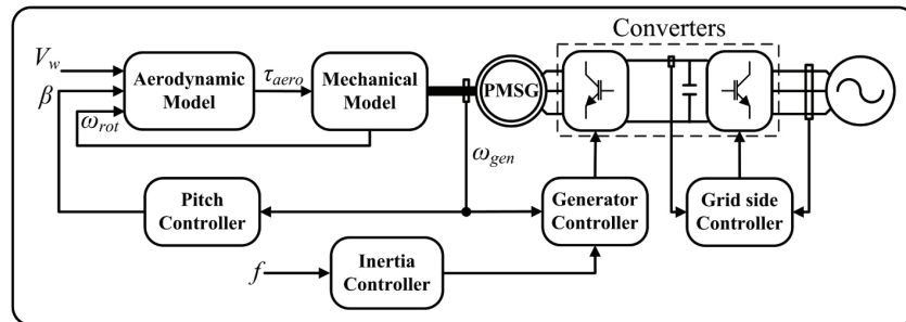
Figure 1: Block diagram of the PMSG-FRPC based wind turbine implemented in Simulink
