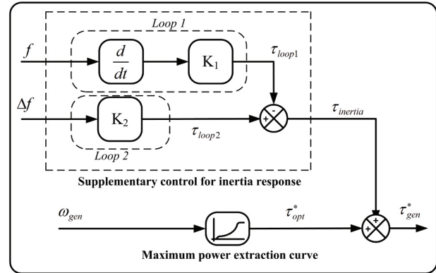
Figure 2: Inertia control loops [8]
