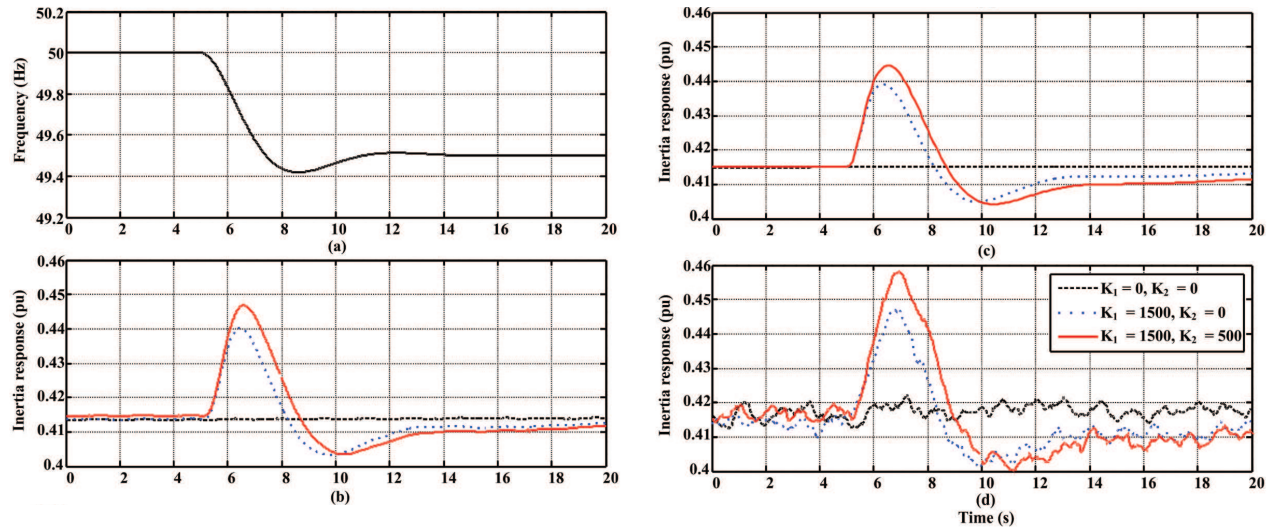
Figure 7: Inertia response (a) frequency deviation; (b) simulation- detailed model; (c) simulation - simplified model; (d) experiment (all values are with respect to the machine base)
