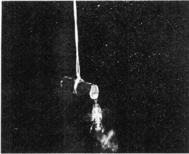
Fig. 2.: A. koschevnikovi drone attracted to the standard dummy. A section of black pencil (length 34 mm, diameter 8 mm) was tied to a thread and impregnated with 1 mg 9-ODA.
