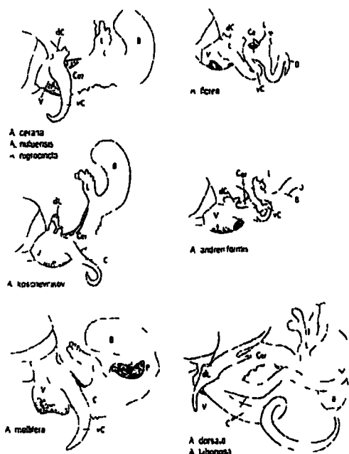
Figure 4. Everted endophalli of nine Apis species (lateral view). Symbols for all figures: B: bulbus; Cer: cervix; P: chitinous plate of bulb; dk: dorsal cornus; l: lobe; V: vestibulum; cc: ventral cornua; &#246;: hairy bulb.
