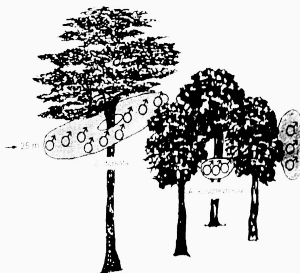
Fig. 1: Drone congregation areas in Sabah (Borneo). A. dorsata drones congregated directly under the canopy of high emergent trees. A. koschevnikovi drones congregated under the thick cover of branches and trees. A. cerana drones remained near the branches of neighbouring vegetation. All three drone congregation areas were within a distance of 30 m. ♂ Spaces occupied by drone flight.
