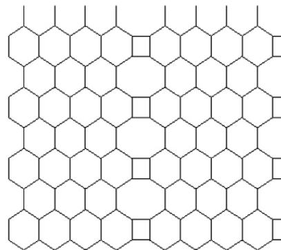
Figure 6: The 2-D graph lattice of L = L[p,q] with p = 2 and q = 4
