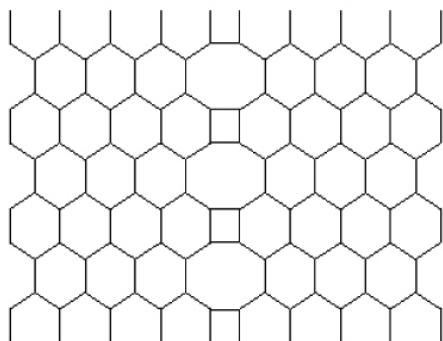
Figure 5: The 2-D graph lattice of K = K[p,q] with p = 2 and q = 3
