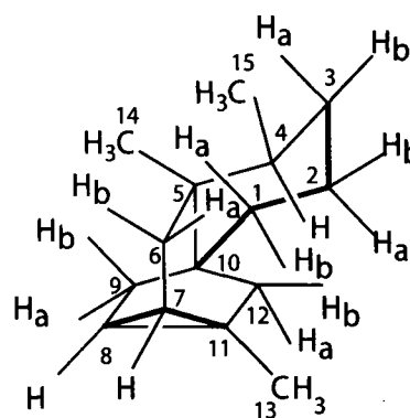
Figure 1: Ishwarane (numbering of carbons according to Joulain and Konig 18 )
