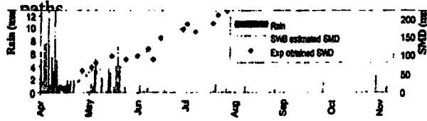
Fig.6. Experimental soil moisture deficit and soil water balance model estimated soil moisture deficit
