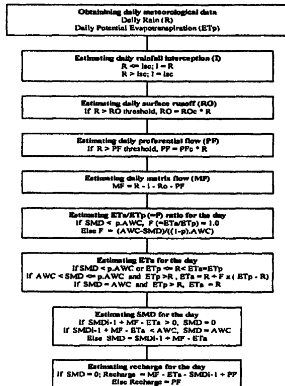
Fig. 5. Flow chart of the soil water balance model suitable for the dry zone of Sri Lanka.
