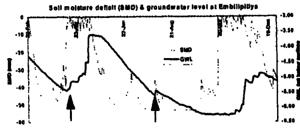
Fig.4. Groundwater level at Embilipitiya with soil moisture deficit in 1995 (after de Silva 1996).
