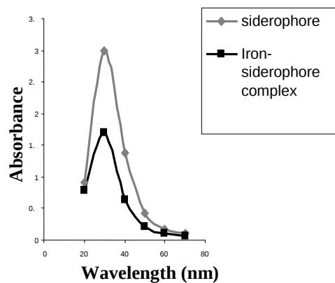
2B. Scan of Iron and Iron- Siderophore complex
