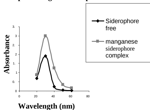
2G. Scan of Manganese and siderophore-Mn complex
