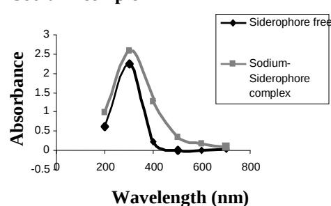
2N. Scan of Sodium and Siderophore-Sodium complex
