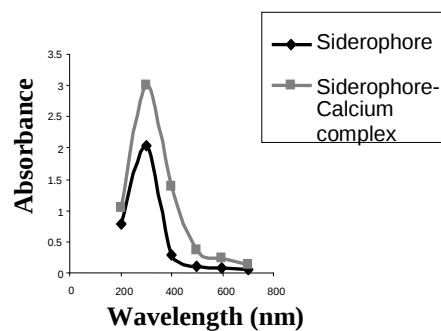
2D. Scan with Calcium and Calcium-Siderophore complex
