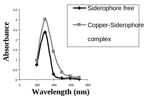
2E. Scan with copper and siderophore-copper complex
