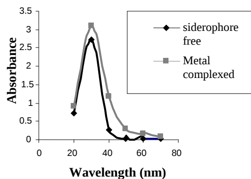
2H. Scan of Mercury and Mercury-siderophore complex
