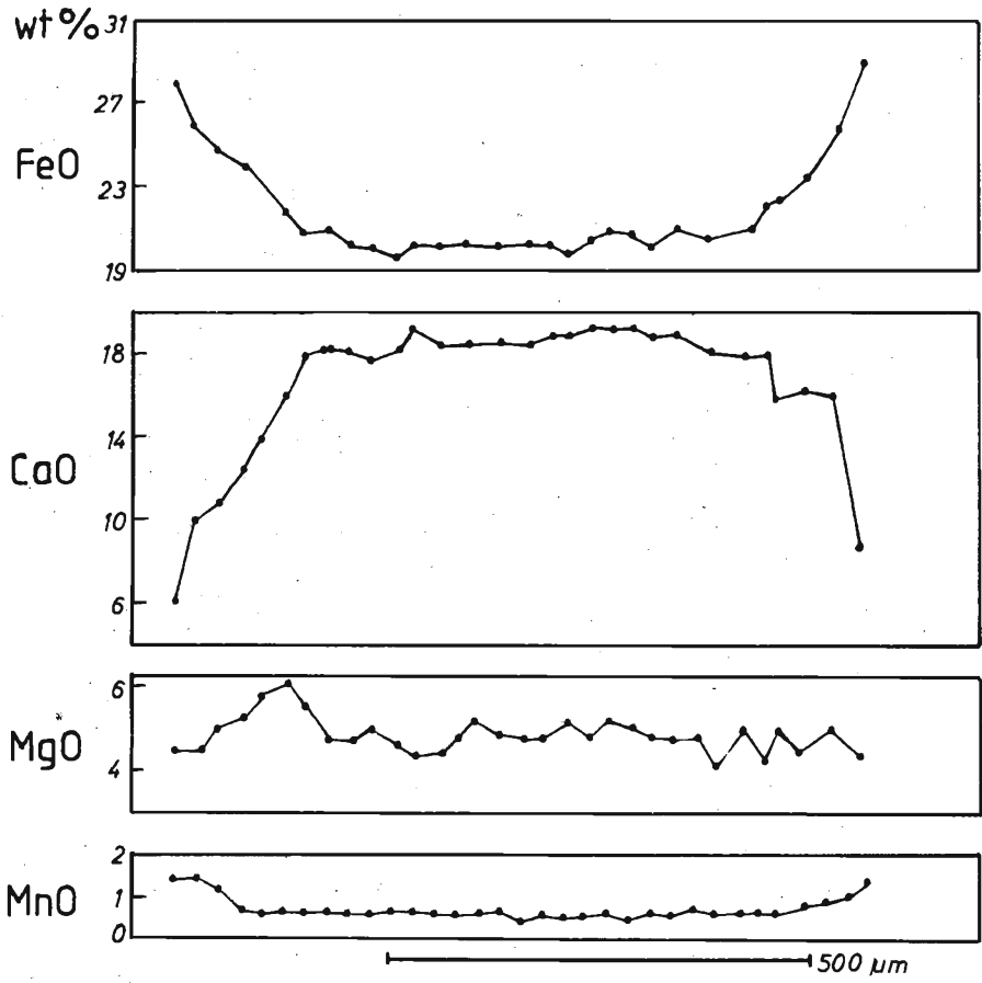
Figure 3c. Compositional profiles of a garnet in a pyroxene granulite
