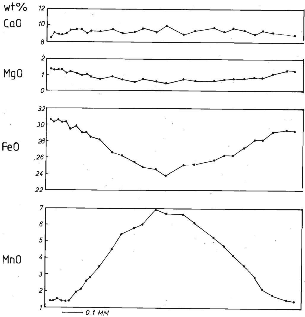
Figure 3a. Compositional profiles of a garnet in the albite schist.
