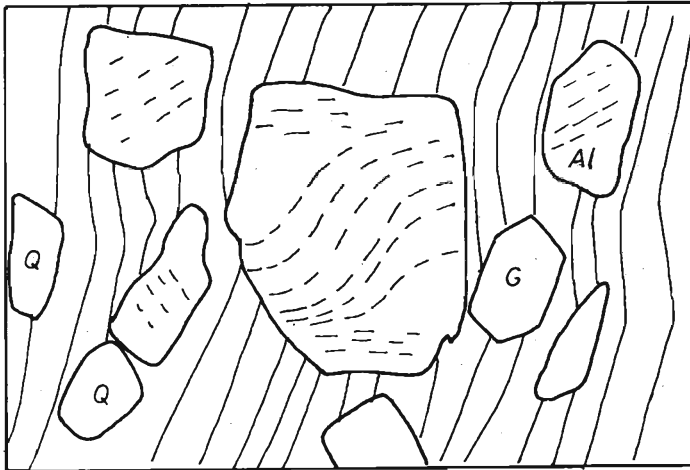
Figure 2a. Albite microporphyroblasts containing numerous oriented inclusions. Note the crenulation of the S-surface, Al-albite, G-garnet, Q-quartz. Phyllosilicates form the S-surface.
