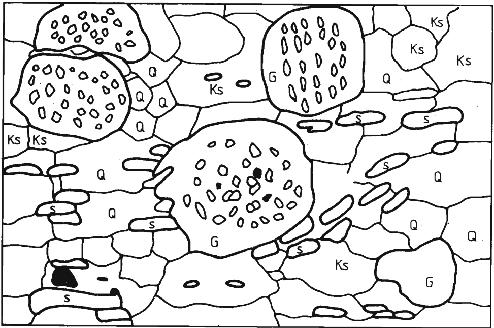
Figure 2b. Subrounded garnets containing a large inclusion-rich core and a narrow inclusion-free rim (garnet-sillimanite schist) KS-micropertite, Q-quartz, S-sillimanite.
