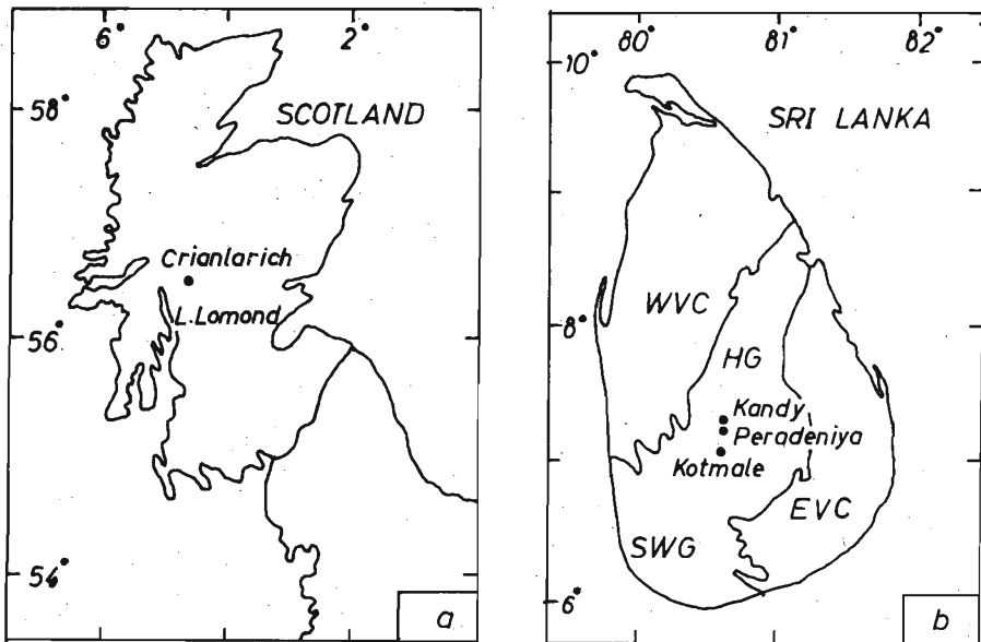
Figure 1. (a) Map of Scotland showing the sample locations. (b) Simplified geological map of Sri Lanka and the sample locations.
