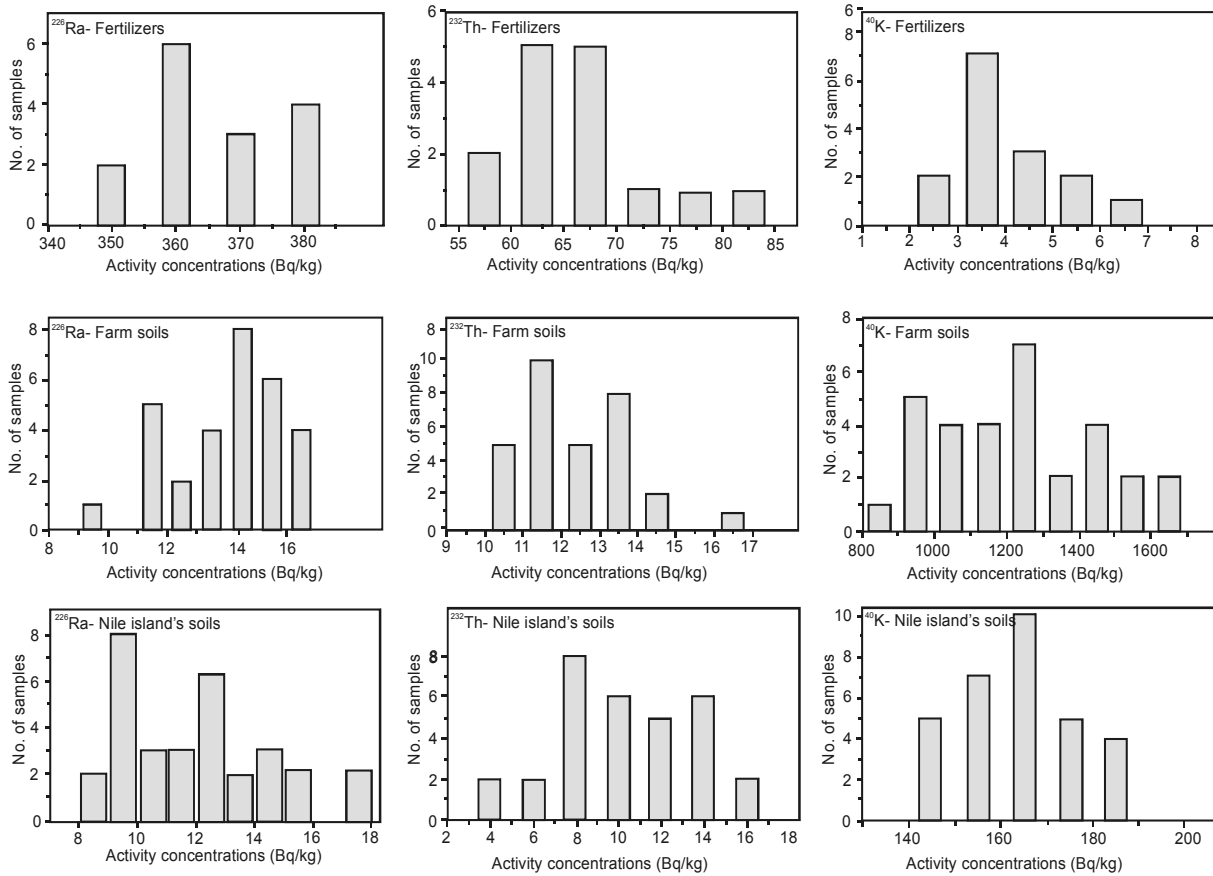
Figure 4: Distribution of 226 Ra, 232 Th and 40 K in phosphate fertilizers, farm soils and Nile island's soils 30
