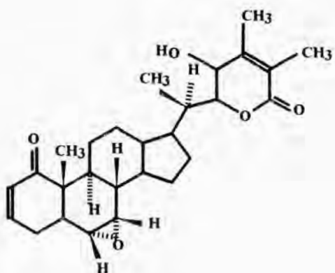
5- dehydroxy withasomnilide
