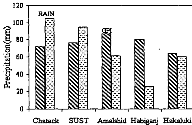
Figure 3. Same as Figure 2 except for 3-days
