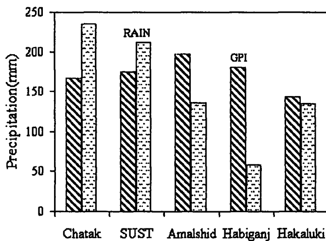
Figure 4. Same as Figure 2 except for 7-days.
