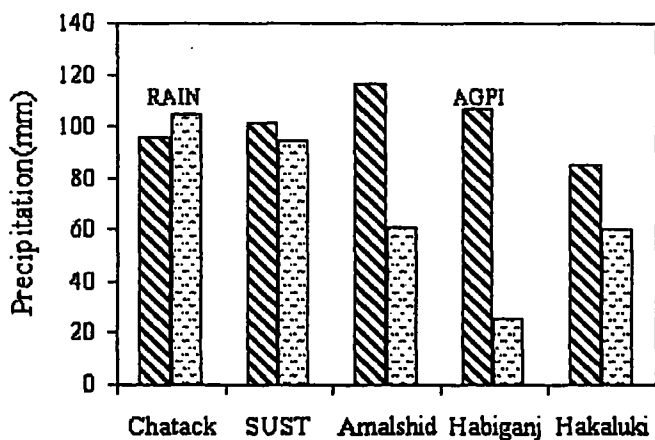
Figure 6. Same as Figure 3 except for AGPI I
