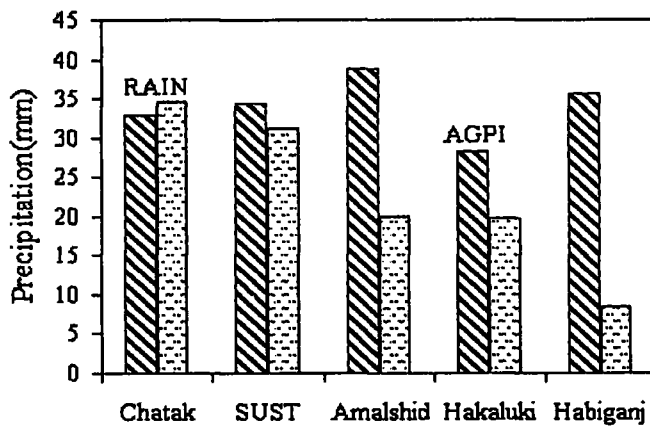
Figure 5. Same as Figure 2 except for AGPI.
