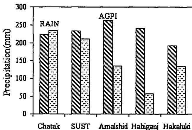
Figure 7. Same as Figure 4 except for AGPI
