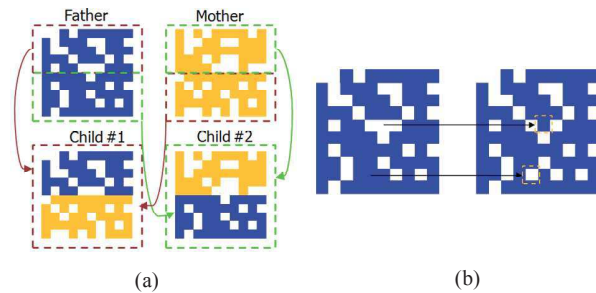
Figure 5: GA operations (a) Crossover (two children are generated from their parents); (b) Mutation (few bits are mutated)
