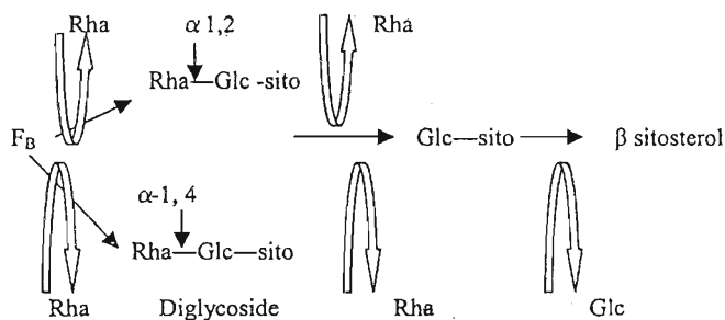
Figure 4: Proof of Branched Structure of F_B
