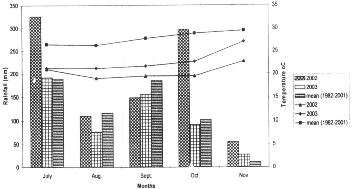
Fig. 1 Monthly rainfall and mean monthly temperatures for 2002, 2003 and mean of 1982-2001 during the late rainy season cropping
