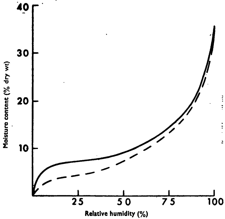
FIG. 4—Diagrammatic representation of moisture sorption by Dust at 32°C—Unbroken line—desorption, broken line—adsorption.
