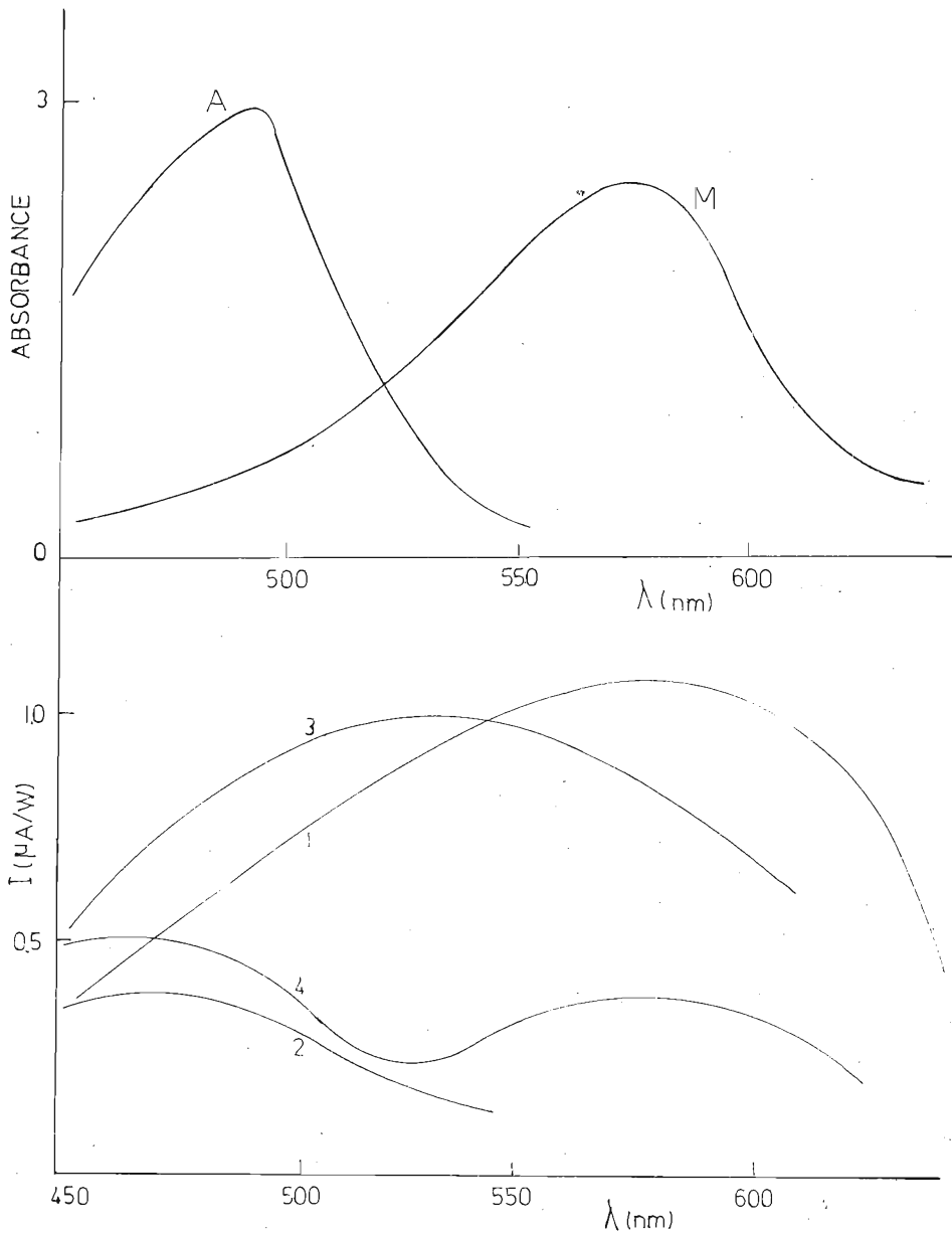
Figure 1. Photocurrent spectrum of cells sensitized with (1) Methyl Violet (2) Acridine Orange (3) Acridine Orange on Methyl Violet (4) Mixture of Acridine Orange and Methyl Violet for comparison the fluorescence spectrum of Acridine Orange and the absorption spectrum of Methyl Violet are indicated above.
