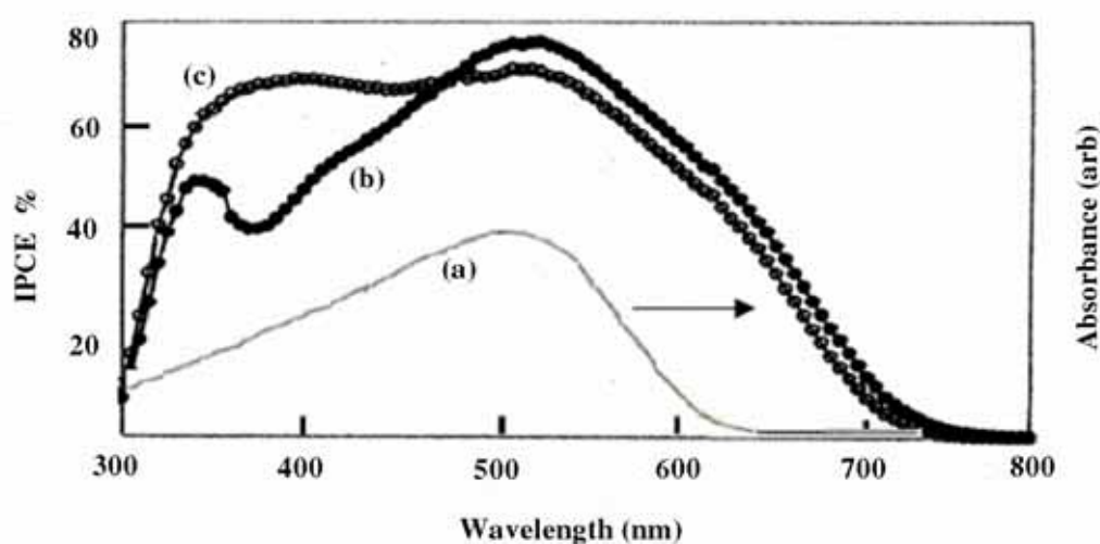
Fig 4. The UV-visible absorption spectrum of the dye in ethanol (a) and the photocurrent action spectra of the cells employing either the HMIIm/ \text{I}_2 /LiSCN electrolyte (b) or the liquid electrolyte (c).
