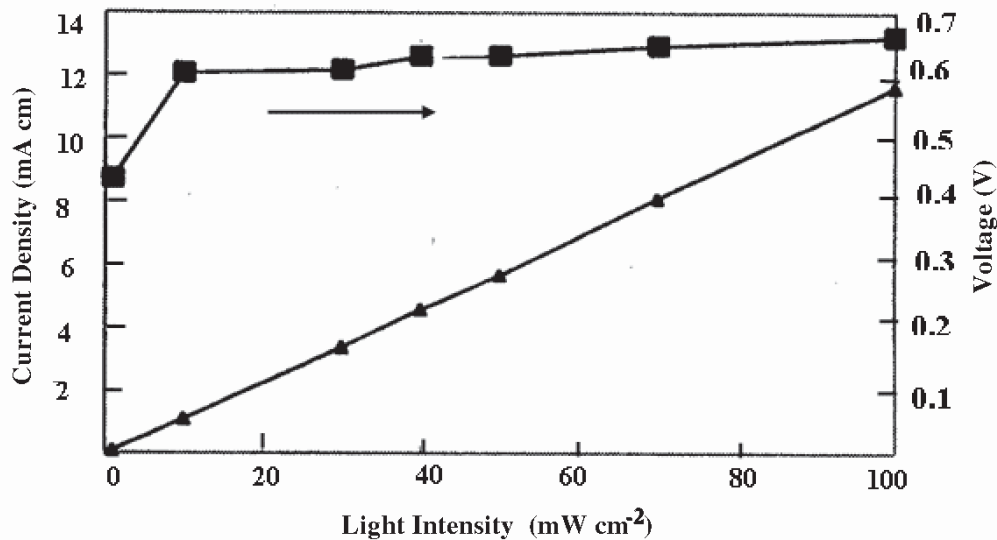
Fig. 3 Incident light dependence of the cell parameters ( J_{sc} and V_{oc} ) of the cell with HMIm/ \text{I}_2 /LiSCN electrolyte.
