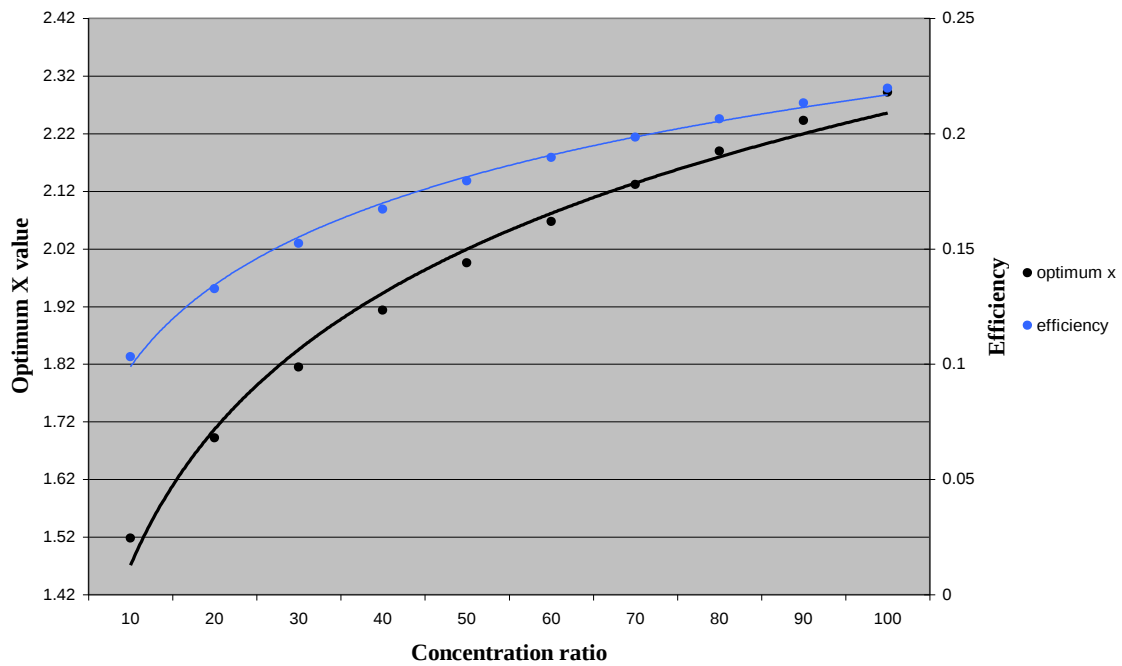
Fig. 4 The graph of second maximum efficiency \eta_{max,max} and x_{opt,opt} as a function of concentration ratio C_n for a classical thermodynamic model for f = 1.03 & s = 10 .
