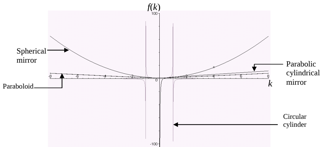
Fig. 5 Shape factors of different type of mirrors
