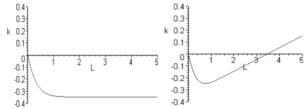
Figure 4: (a) k is \approx -0.38 when \alpha \rightarrow 1 Figure 4: (b) \alpha increased
