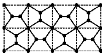
Figure 1: Pentagonal lattice with nearest neighbour interactions
