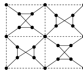
Figure 2: Star-triangle transformation for pentagonal lattice
