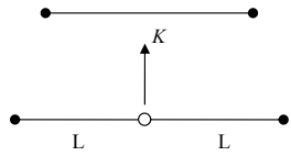
Figure 3: Effective coupling k
