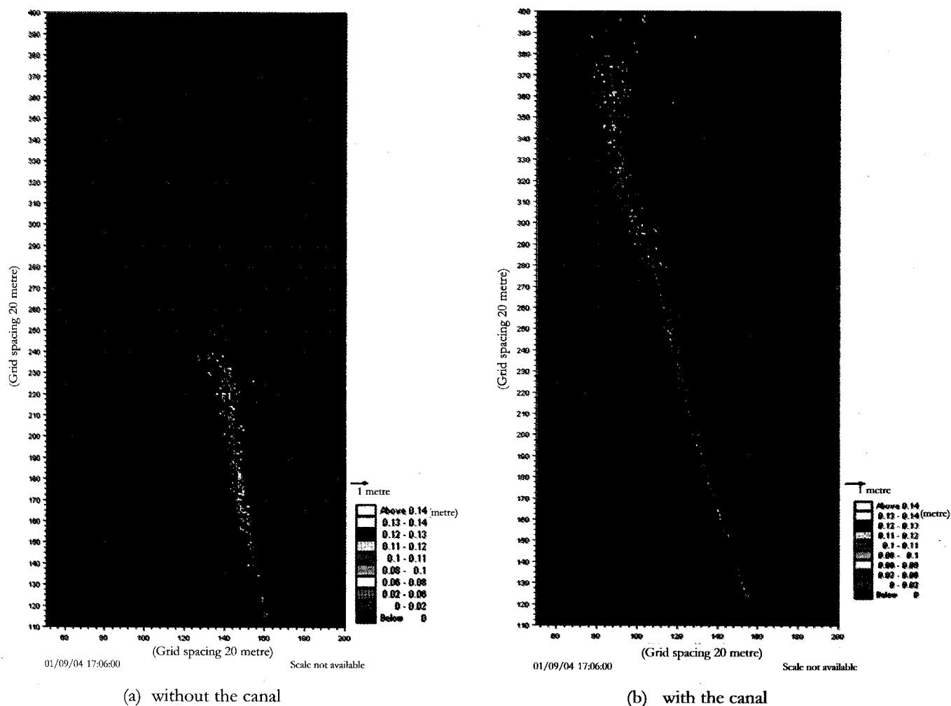
Figure 5: Dispersal of dredged mud (30 \mu\text{m} ) during dredging 14.75 m/s wind from South West
