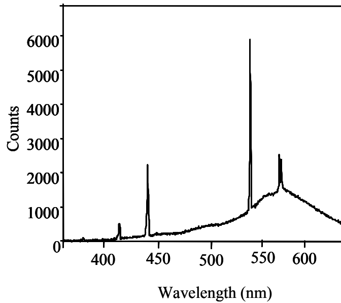
Figure 2: Calibration lines arising from Hg emission by a fluorescent lamp 20 W Philips
