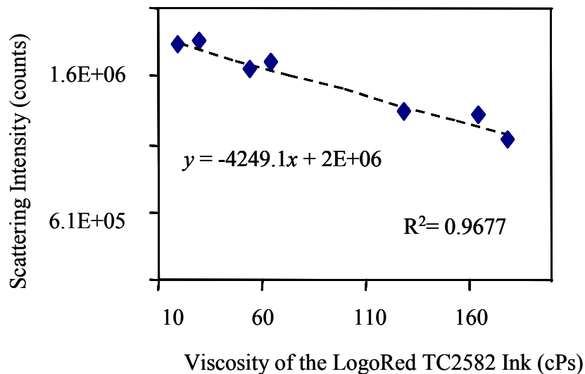
Figure 5: Plot of ink viscosity and scattered intensity of the light for the letter “J”
