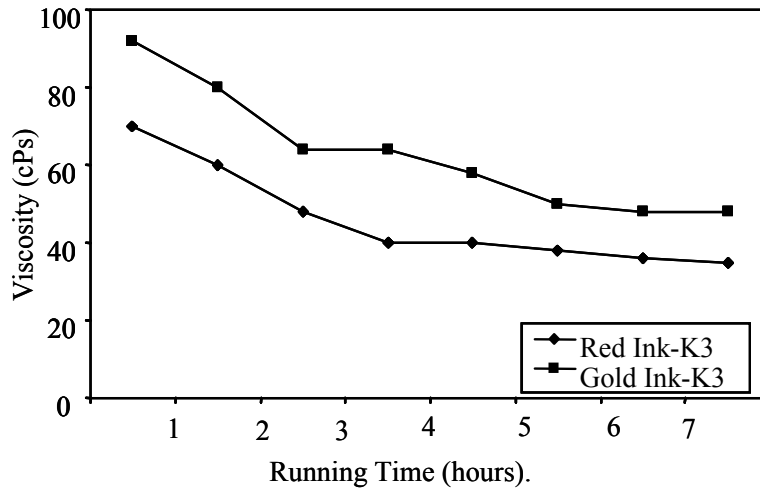
Figure 4: Variation of ink viscosity with the running time of the K3 machine
