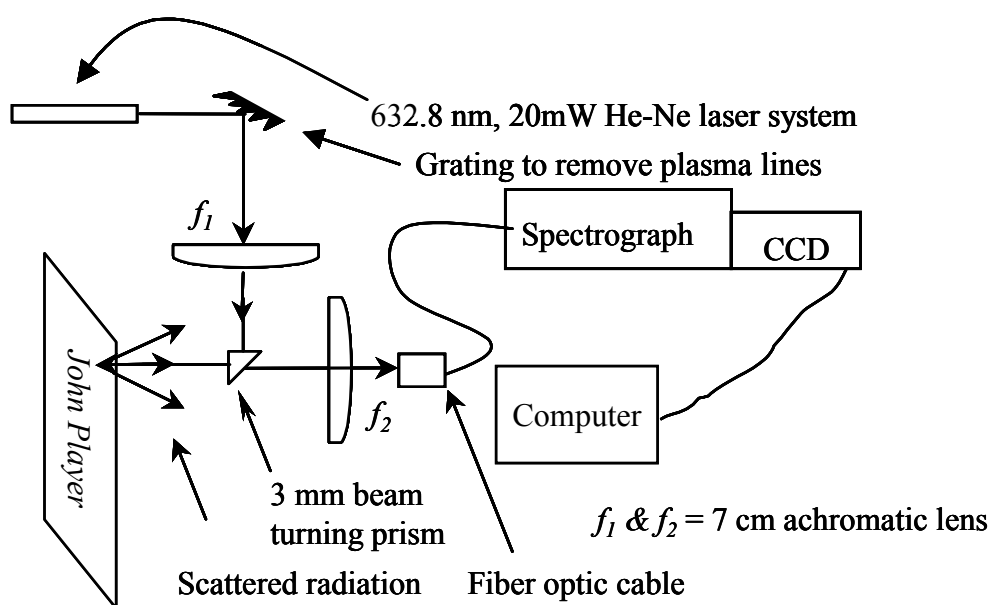
Figure 1: Experimental set-up assembled to examine the viscosity and scattering intensity relationship
