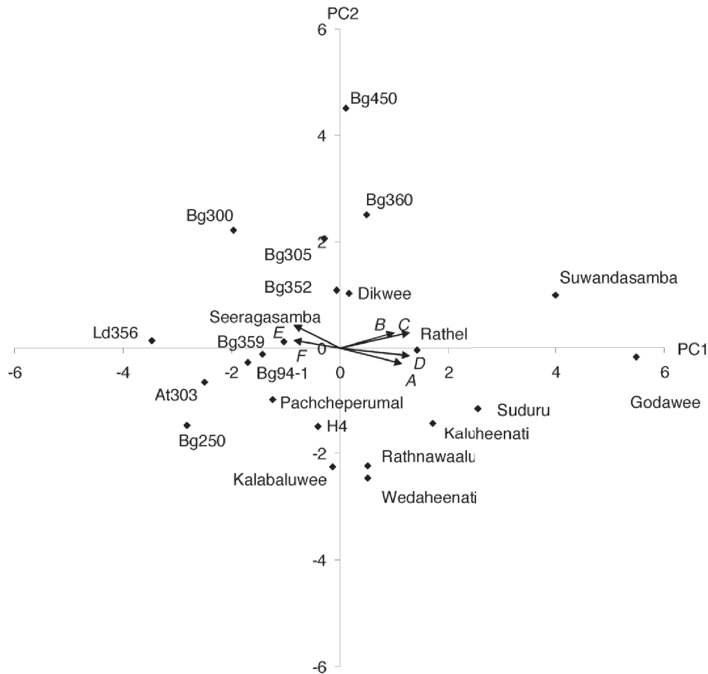
Figure 1: Score plot of PC1 versus PC2 of rice varieties based on vegetative and reproductive characteristics. The vectors represent the variable loadings; A- plant height, B- leaf area at heading, C- leaf DW at heading, D- stem DW at harvesting, E- total grains panicle -1 and, F- filled grains panicle -1 .
