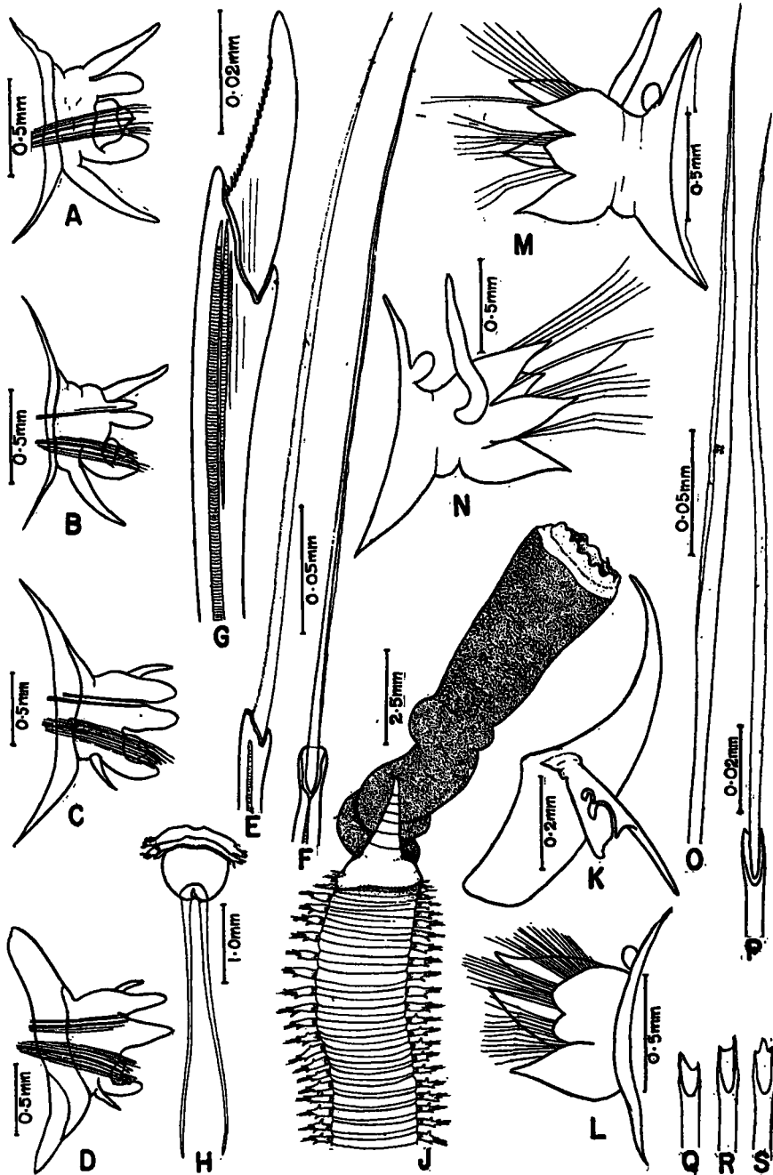
TEXT-FIGURE 3.— Perineris nuntia (Sav.) var. vallata Grube, A—H. A, Anterior view of first left foot; B, Anterior view of third left foot; C, Anterior view of 10th left foot; D, Anterior view of 25th left foot; E & F, Homogomph spinigers; G, Heterogomph falciger; H, Anal segment. Glycera rouxii Audouin and Milne Edwards, J—S. J, Dorsal view of anterior end, with everted proboscis; K, A jaw from the proboscis; L, Posterior view of 10th left foot; M, Posterior view of an extreme posterior left foot; N, Anterior view of an extreme posterior left foot; O, Dorsal seta; P, Ventral seta; Q—S, Variations of the articular joints of the ventral setae.
