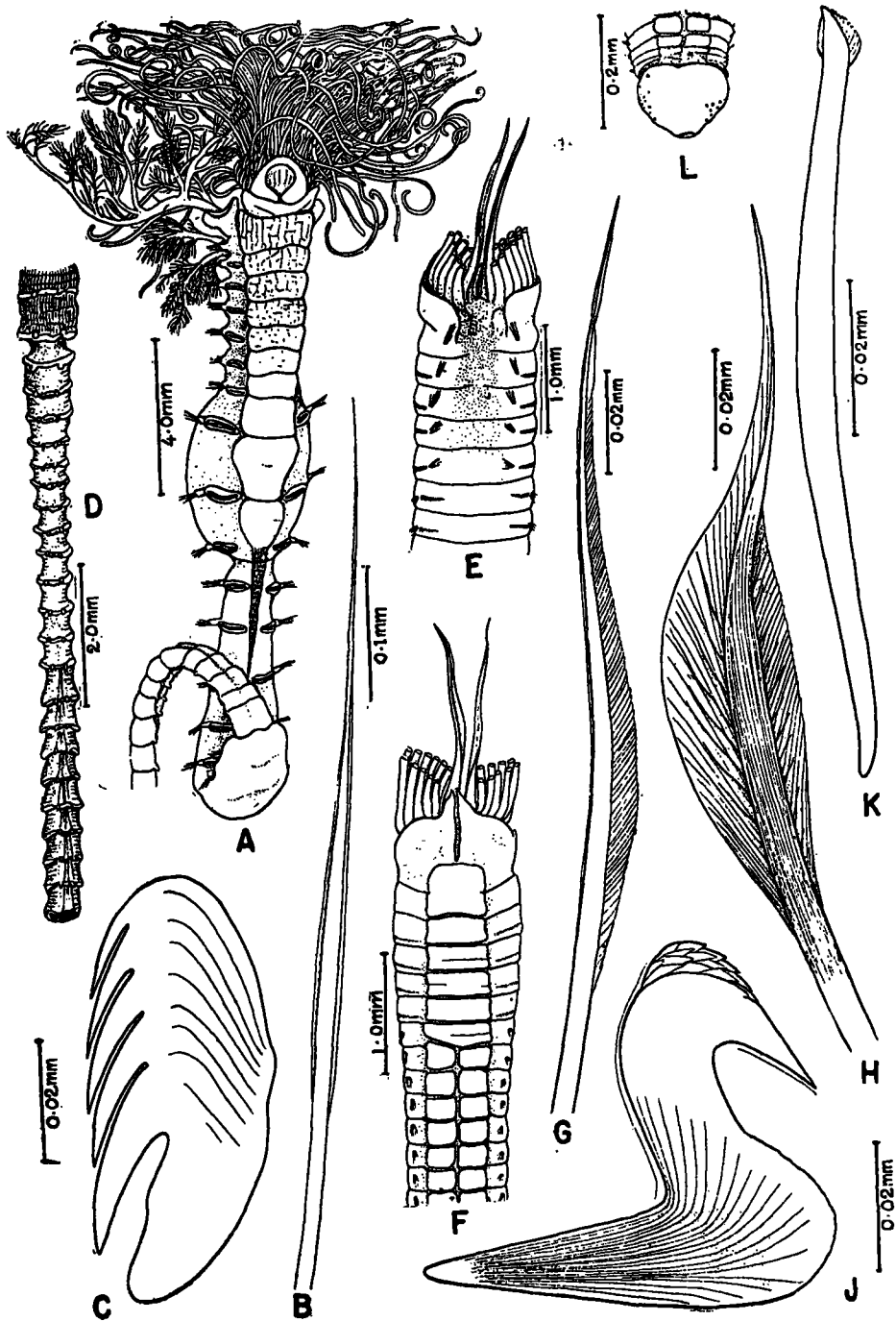
TEXT-FIGURE 11.— Loimia decora , sp. nov., A—D. A, Ventral view of the thorax and a few abdominal segments; B, Notopodial seta from the first foot; C, Uncinus from the 3rd thoracic neuropodial torus; D, Ventral view of 63rd and 64th feet and the rectal tube. Potamilla brevithoracica , sp. nov., E—L. E, Dorsal view of anterior end (gill pinnules not shown); F, Ventral view of anterior end (gill pinnules not shown); G, Notopodial seta from the first thoracic setigerous segment; H, Paddle-shaped seta from the 2nd thoracic notopodial bundle; I, Thoracic hook (uncinus); J, Pennoned (pickaxe shaped) seta from a thoracic neuropodial torus; K, Pennoned (pickaxe shaped) seta from a thoracic neuropodial torus; L, Dorsal view of anal segment.
