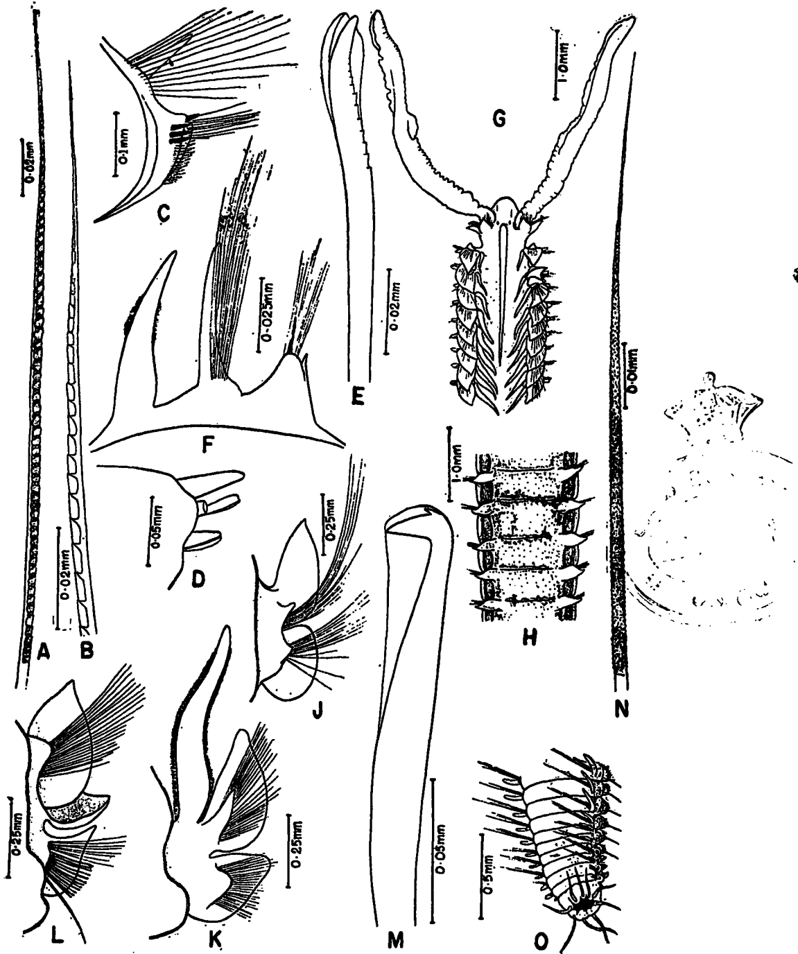
TEXT-FIGURE 8.— Scoloplos (Leodanus) gracilis , sp. nov., A—F. A, Thoracic notopodial seta; B, Thoracic neuropodial seta; C, Anterior view of 5th left foot; D, Dorsal part of thoracic neuropodial ramus, showing aciculum and acicular setae; E, Neuropodial thoracic hook; F, Anterior view of a posterior abdominal foot. Laonice brevicristata , sp. nov., G—O. G, Dorsal view of anterior end; H, Dorsal view of 60th—64th feet; J, Anterior view of first left foot; K, Anterior view of 25th left foot; L, Anterior view of 45th left foot; M, Ventral hook from the 45th foot; N, Stout, ventral seta from a posterior foot; O, Dorso-lateral view of posterior end.
