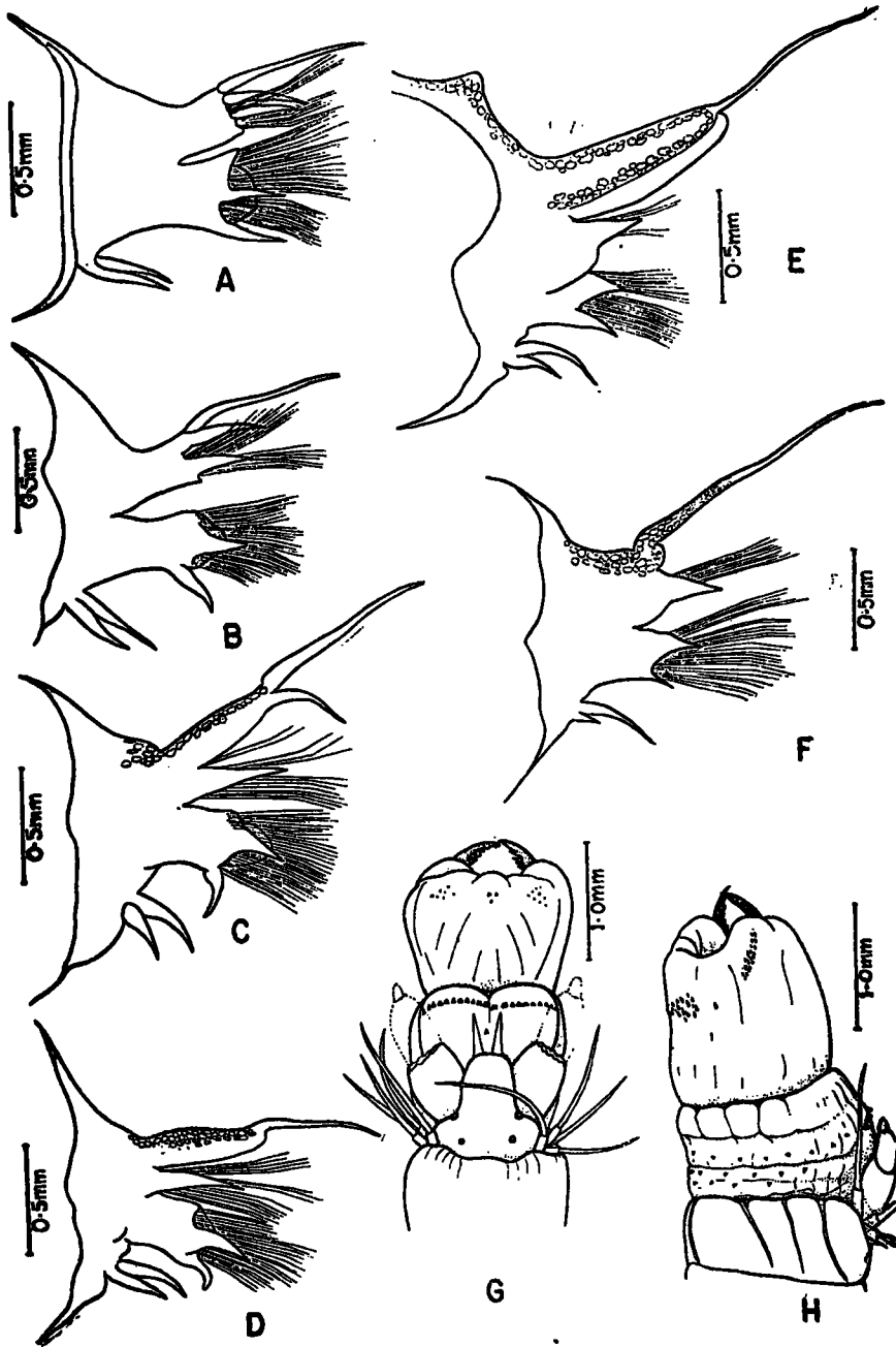
TEXT-FIGURE 2.— Tambalagania fauveli , gen. et sp. nov., A—F. A, Anterior view of 10th left foot; B, Anterior view of 14th left foot; C, Anterior view of 15th left foot; D, Anterior view of 16th left foot; E, Anterior view of 40th left foot; F, Anterior view of 70th left foot. Perinereis muntia (Sav.) var. vallata Grube, G—H. G, Dorsal view of prostomium and proboscis; H, Left lateral view of proboscis.
