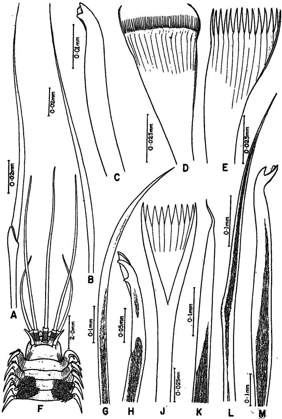
TEXT-FIGURE 5.— Marphysa sanguinea (Mont.), A—E. A, Ventral compound seta from the 47th foot; B, Simple, flattened dorsal seta; C, Ventral hook from the 360th foot; D, Comb seta from the 300th foot; E, Comb seta from the 360th foot. Diopatra neapolitana Delle Chiaje, F—M. F, Dorsal view of anterior end; G, Dorsal seta from the first foot; H, Ventral, pseudocompound seta from the first foot; J, Comb seta from the 5th foot; K, Tip of an aciculum; L, Ventral seta from the 50th foot; M, Ventral hook from the 50th foot.
