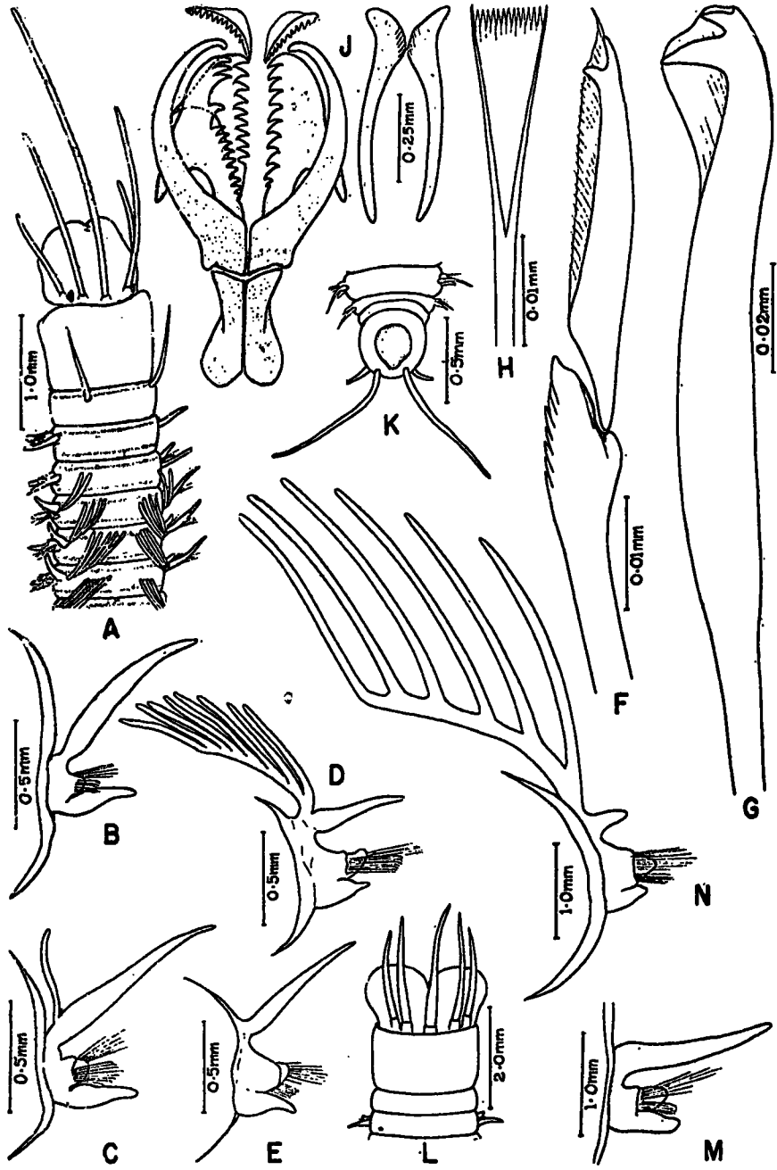
TEXT-FIGURE 4.— Eunice savignyi Grube, A—K. A, Dorsal view of anterior end; B, Anterior view of first left foot; C, Anterior view of 3rd left foot; D, Anterior view of 20th left foot; E, Anterior view of 30th left foot; F, Compound ventral seta from the first foot; G, Bidentate acicular hook from the 65th foot; H, Comb seta from the 30th foot; J, Dental apparatus (dorsal view); K, Dorsal view of anal segment. Marphysa sanguinea (Mont.), L—N. L, Dorsal view of anterior end; M, Anterior view of first left foot; N, Anterior view of 153rd left foot.
