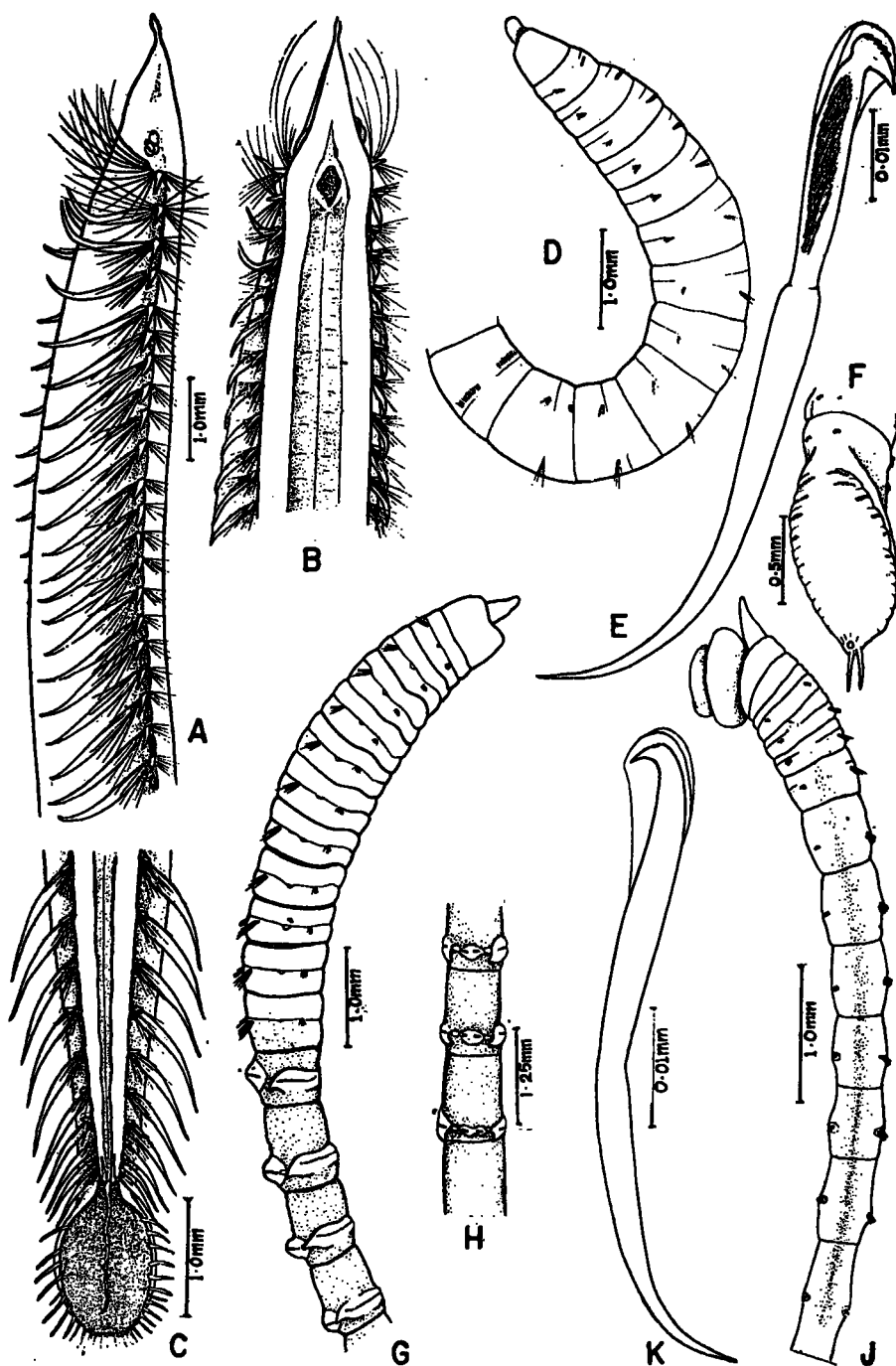
TEXT-FIGURE 9.— Ammotrypane grandis , sp. nov., A—C. A, Lateral view of anterior end; B, Ventral view of anterior end; C, Ventral view of posterior end. Heteromastix platyproctus , sp. nov., D—F. D, Lateral view of anterior end; E, Abdominal hook; F, Dorsal view of posterior end. Notomastus ceylonicus , sp. nov., G—H. G, Lateral view of anterior end; H, Dorsal view of 8th—10th abdominal segments. Heteromastus deductus , sp. nov., J—K. J, Lateral view of anterior end, with everted proboscis; K, Abdominal hook.
