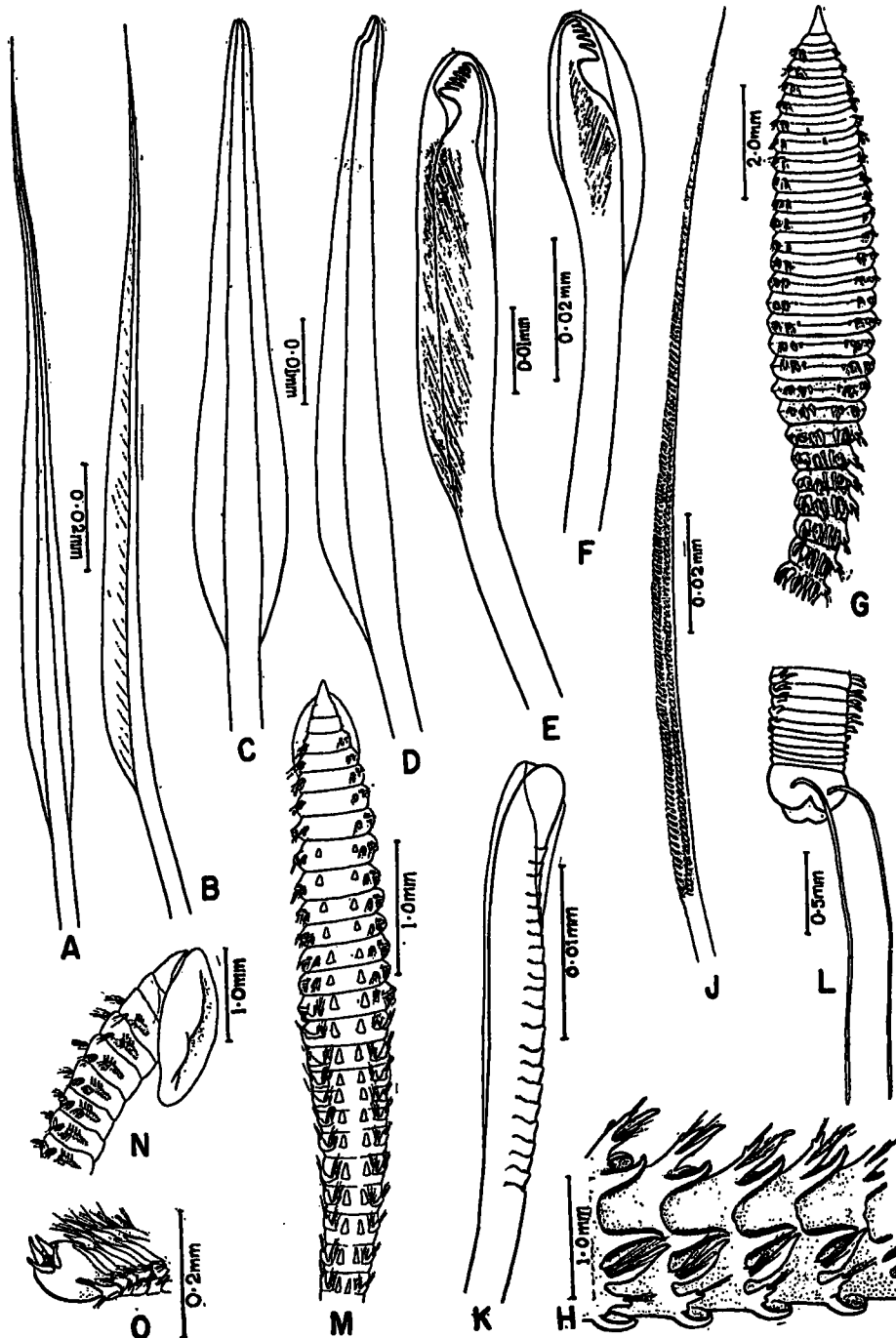
TEXT-FIGURE 7.— Lumbrineris emandibulata , sp. nov. A—F. A, Dorsal seta from the first foot; B, Same seta in side view; C, Seta from the middle group of the first foot; D, Same seta in side view; E, Hook, with long guard, from the 20th foot; F, Hook, with short guard, from the 26th foot. Scoloplos (Scoloplos) marsupialis Southern, G—L. G, Dorsal view of anterior end; H, Lateral view of a few abdominal segments showing the pockets; J, Dorsal thoracic seta; K, Ventral hook from the 6th foot; L, Dorsal view of anal segment. Scoloplos (Leodanus) gracilis , sp. nov., M—O. M, Dorsal view of anterior end, with extruded proboscis; N, Lateral view of anterior end, with extruded proboscis; O, Lateral view of anal segment.
