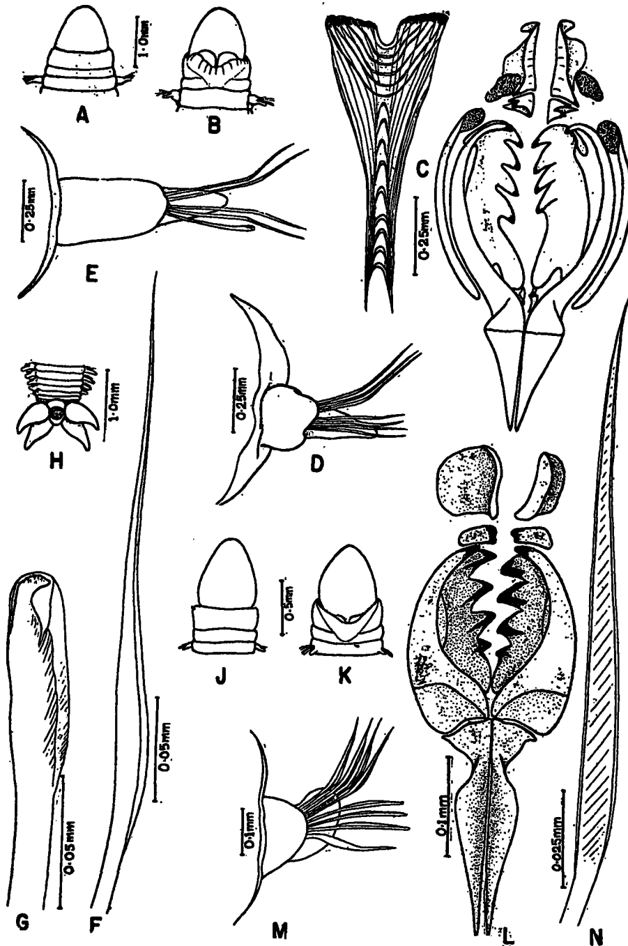
TEXT-FIGURE 6.— Lumbrineris pseudopolydesma , sp. nov. A—H. A, Dorsal view of anterior end; B, Ventral view of anterior end; C, Dental apparatus (dorsal view); D, Anterior view of first left foot; E, Anterior view of a foot from the middle of the body; F, Seta from the 54th foot; G, Ventral hook from the 54th foot; H, Dorsal view of anal segment. Lumbrineris emandibulata , sp. nov. J—M. J, Dorsal view of anterior end; K, Ventral view of anterior end; L, Dental apparatus (dorsal view); M, Anterior view of 10th left foot; N, Ventral seta with flattened blade from first foot.
