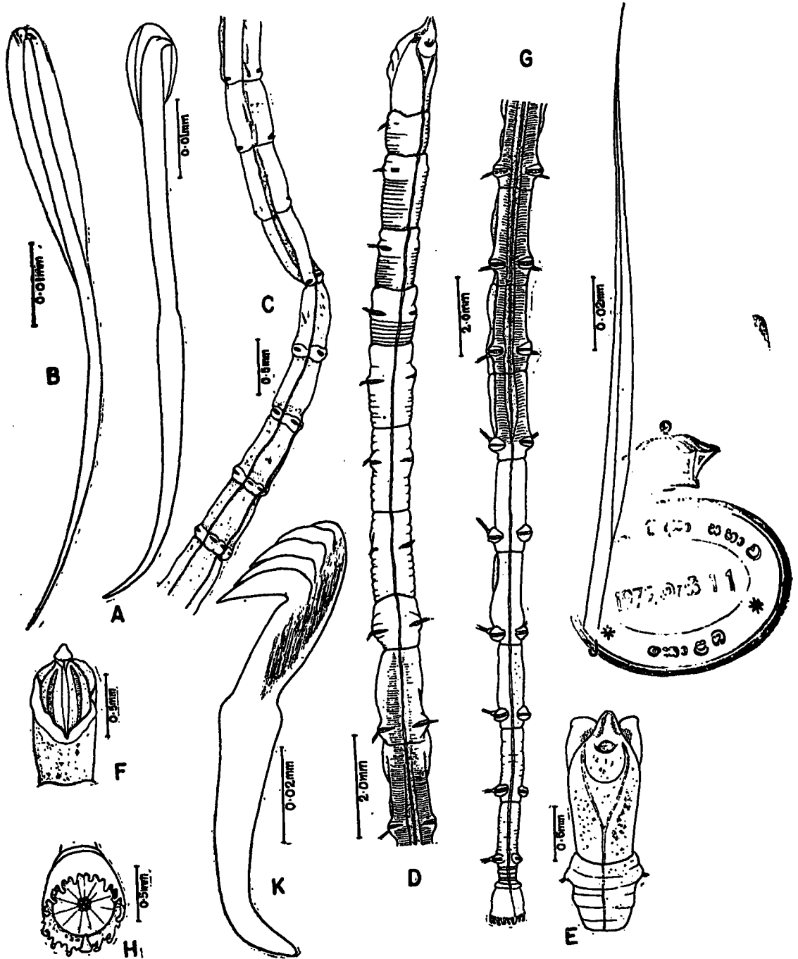
TEXT-FIGURE 10.— Notomastus ceylonicus , sp. nov., A, Abdominal hook. Heteromastus deductus , sp. nov., B—C. B, Long, stalked thoracic hook; C, 27th—34th abdominal segments. Axiothella tambalagamensis , sp. nov., D—K. D, Ventral view of prostomium, buccal segment and 1st—10th setigerous segments; E, Ventral view of prostomium, buccal segment and first setigerous segment; F, Dorsal view of cephalic plate; G, Ventral view of 10th—18th setigerous segments and the anal funnel; H, Postero-dorsal view of the anal funnel; I, Notopodial seta from the first foot; J, Hook from the 8th foot. K, Hook from the 8th foot.
