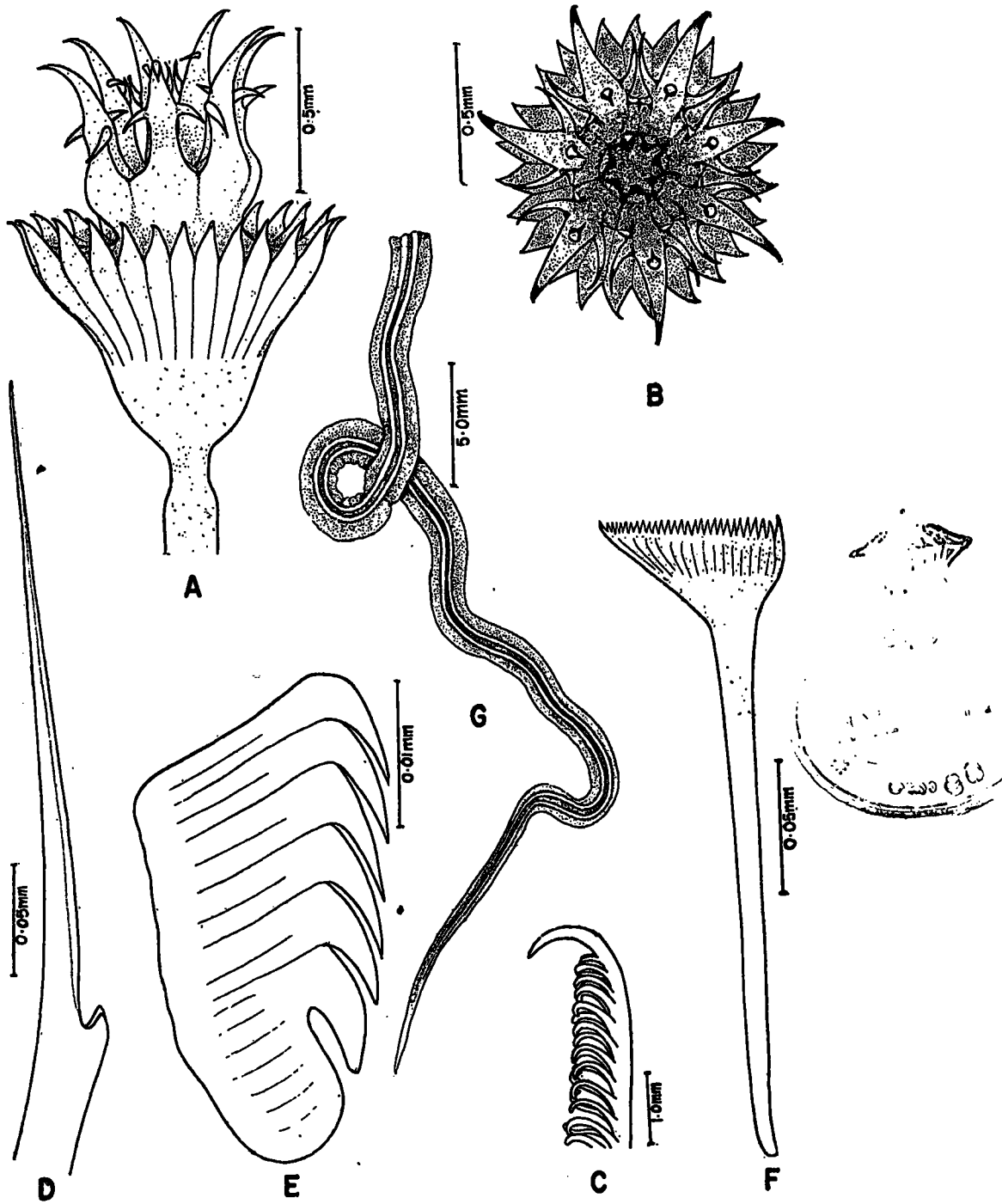
TEXT-FIGURE 12.— Hydroides tambalagamensis , sp. nov., A—G. A, Lateral view of operculum; B, Top view of operculum; C, Tip of a gill; D, Bayonet-shaped collar seta; E, Thoracic uncinus; F, Anterior abdominal seta; G, Tube.
