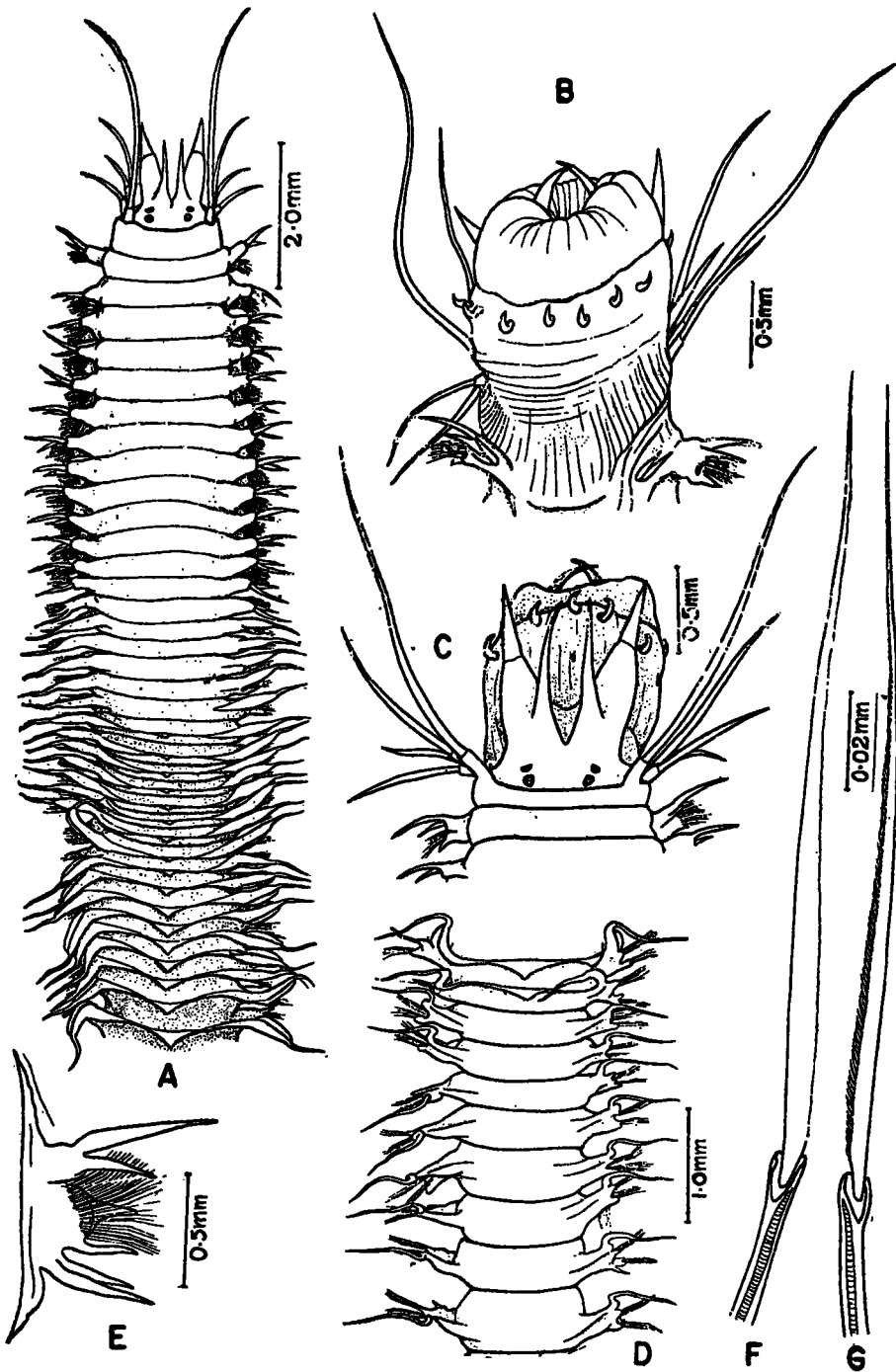
TEXT-FIGURE 1.— Tambalagania fauveli , gen. et sp. nov., A—G. A, Dorsal view of anterior portion of worm; B, Ventral view of proboscis; C, Dorsal view of prostomium and proboscis; D, Dorsal view of 66th—75th setigerous segments; E, Anterior view of first left foot; F, Homogomph spiniger from first foot; G, Homogomph spiniger with long serrations along one edge, from the first foot.
