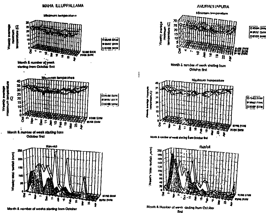
Fig. 1. Minimum and maximum weekly average temperatures and weekly total rainfall prevailed during three consecutive South-west Monsoon (SWM) seasons at Maha Illuppallama and Anuradhapura (1995-98).
