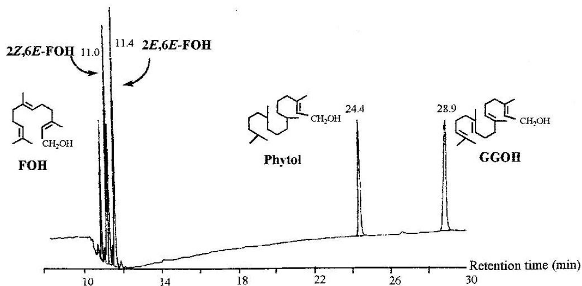
Figure 1. GC Profiles of Authentic Farnesol, Geranylgeraniol and Phytol. (Shimadzu GC 17-A Gas Chromatograph, column- J & W Scientific DB-1, i.d. 0.25 mm x 60 m; initial temp. 60 o C for 5 min, progress rate; 2 o C/min, final temp. 220 o C; carrier gas- He, flow at 1.2 ml/min).
