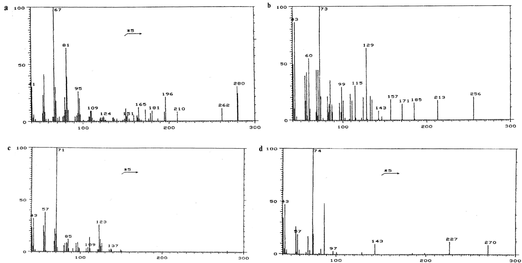
Figure 4. Mass spectra of hydrolysed chloroplast extract of H. planus . a) linoleic acid, b) palmitic acid, c) phytol and d) methyl palmitate. (Hitachi M-80B Gas Chromatograph Column- DB-Wax (i.d. 0.25 mm X 60 m.); initial temp. 60 0 C for 5 min, progress rate 2 0 C/min, final temp. 220 0 C; carrier gas- He, flow rate at 1.1 ml/min;)
