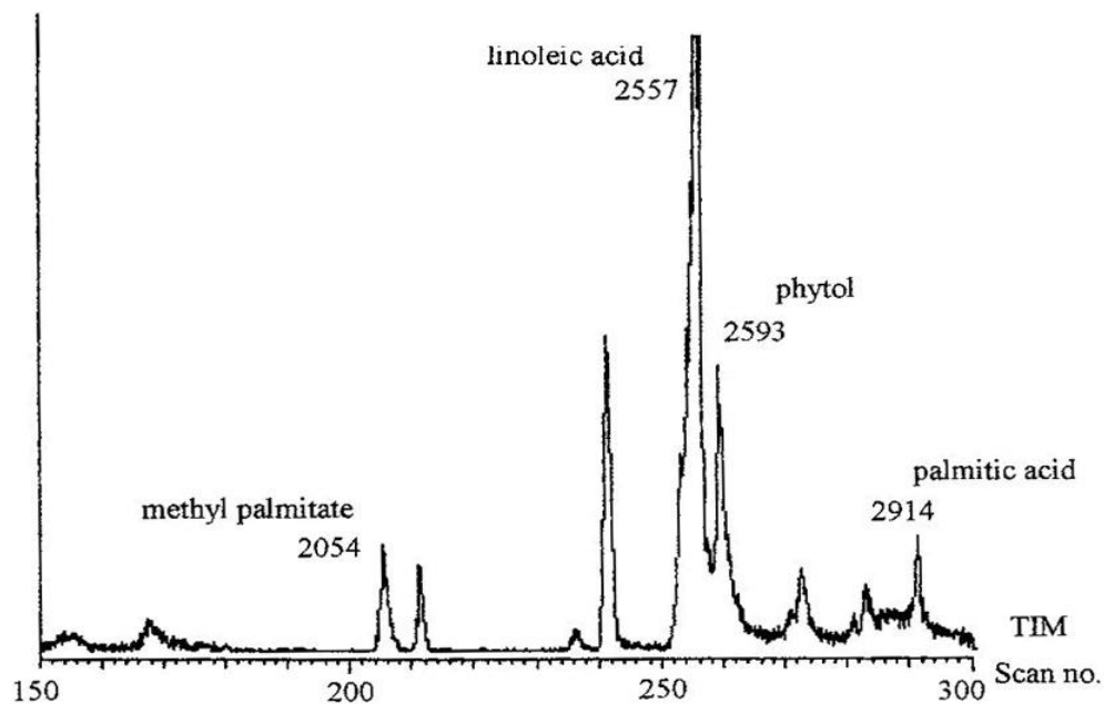
Figure 3. GC-MS profiles of the KOH hydrolysed extract of H. planus intact chloroplasts. (Hitachi M-80B Gas Chromatograph Column- DB-Wax (i.d. 0.25 mm X 60 m,); initial temp. 60 0 C for 5 min, progress rate 2 0 C/min, final temp. 220 0 C; carrier gas- He, flow rate at 1.1 ml/min).
