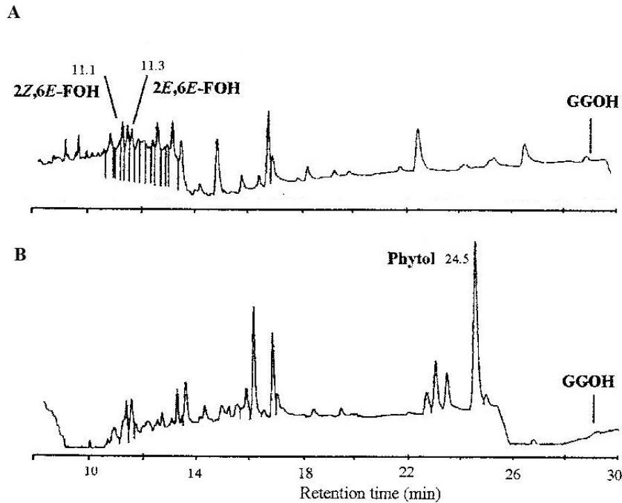
Figure 2. GC profiles of the methanol hydrolysate from intact chloroplasts of H. planus . (Shimadzu GC 17-A Gas Chromatograph, column- J & W Scientific DB-1, i.d. 0.25 mm x 60 m; initial temp. 60 0 C for 5 min, progress rate; 2 0 C/min, final temp. 220 0 C; carrier gas- He, flow at 1.2 ml/min). A) Enzymatic hydrolysis (hydrolysed with 10 \mu l bacterial alkaline phosphatase) and B) KOH hydrolysis (hydrolysed for 2 hrs with 2.5% KOH in methanol under reflux)
