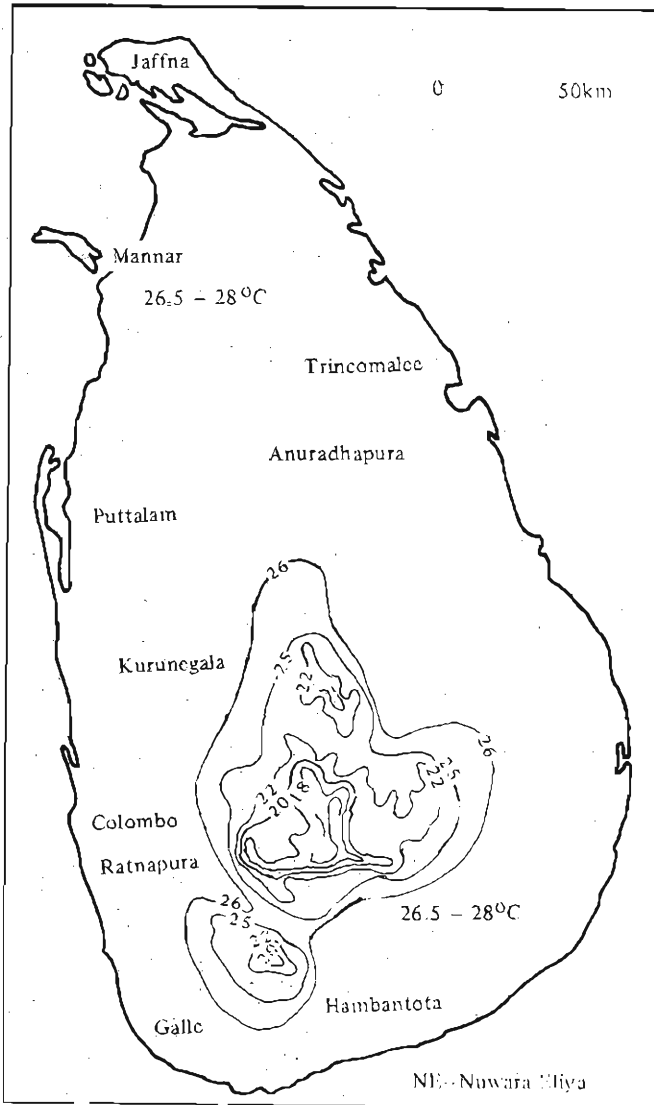
Figure 3 - Map of the annual average temperatures in Sri Lanka, isotherms in °C.
