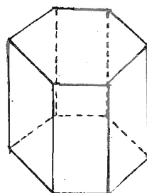
HEXAGONAL
