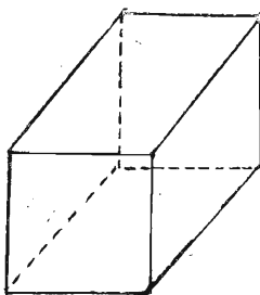
TETRAGONAL
