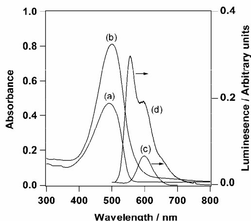
Fig. 1 Absorption spectrum of a MEH-PPV solution in chloroform (a) as obtained (without iodine treatment, 10^{-3} M), (b) after doping iodine in same solution, and emission spectra for MEH-PPV in chloroform different concentrations (c) 10^{-3} M and (d) 10^{-5} M
