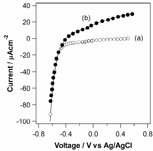
Fig. 2. Current voltage characteristics of a MEH-PPV/TiO 2 electrode (a) at dark and (b) under illumination, in aqueous poly-iodide electrolyte (I - :I 2 =10 5 :1), under three electrode configuration
