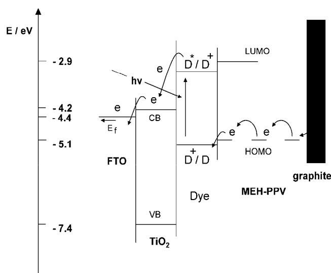
Fig. 6 Electron-transfer process of \text{TiO}_2/\text{N3}/\text{MEH-PPV}/\text{I}_2/\text{graphite} cell where E_f – Fermi Level of FTO, HOMO – highest occupied level of polymer, LUMO – lowest occupied level of polymer, CB – Conduction band of \text{TiO}_2 , VB –Valence band of \text{TiO}_2 , D- ground state of dye molecule, D^* - excited state of dye molecule, D^+ - dye cation
