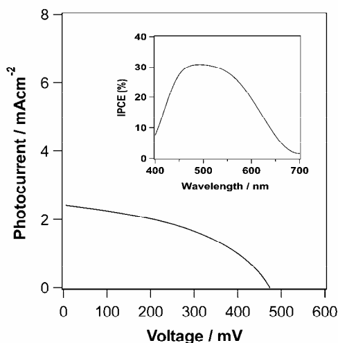
Fig. 5 Current voltage characteristics of \text{TiO}_2|\text{N3}|\text{MEH-PPV}|I_2|\text{graphite} cell under illumination of 100 \text{ mWm}^{-2} . Insert shows the IPCE spectrum of \text{TiO}_2|\text{N3}|\text{MEH-PPV}|I_2|\text{graphite} cell
