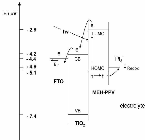
Fig. 3. Band diagram of MEH-PPV/TiO 2 /FTO electrode in polyiodide electrolyte under illumination with flat band concept. Where E_f – Fermi Level of FTO, HOMO – highest occupied level of polymer, LUMO – lowest occupied level of polymer, CB – Conduction band of TiO 2 , VB –Valance band of TiO 2 and E_{redox} – redox potential of poly iodide electrolyte
