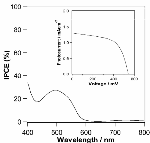
Fig. 4 IPCE spectrum of \text{TiO}_2/\text{MEH-PPV}/\text{polyiodide} cell, Insert shows the current voltage characteristics of the same cell, light intensity is maintained as 100 \text{ mWm}^{-2} , at the electrode surface
