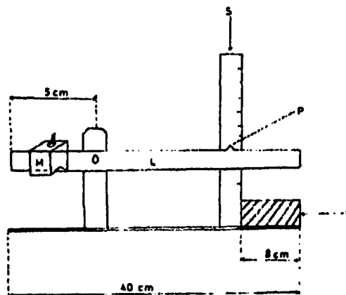
Fig.1 : Husk compression measurement device M- Compression load (= 645.0g), L- Lever, P- Pointer, E-Support, S-Graduated scale
