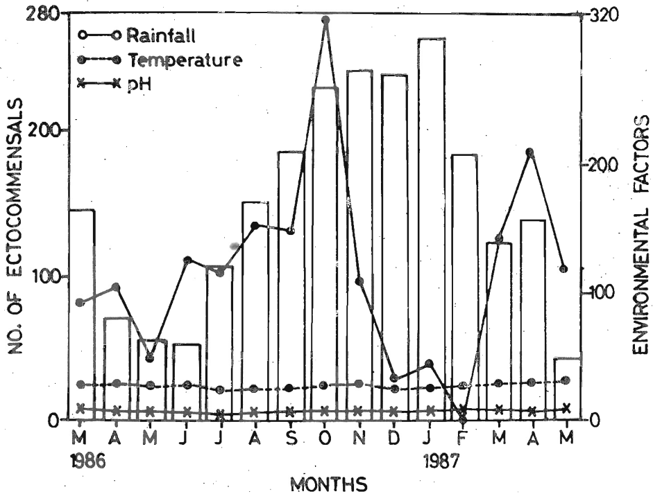
Figure 1: Variation in average water temperature, pH, monthly rainfall and fluctuation in the ecto-commensal population (March 1986 – May 1987.)
