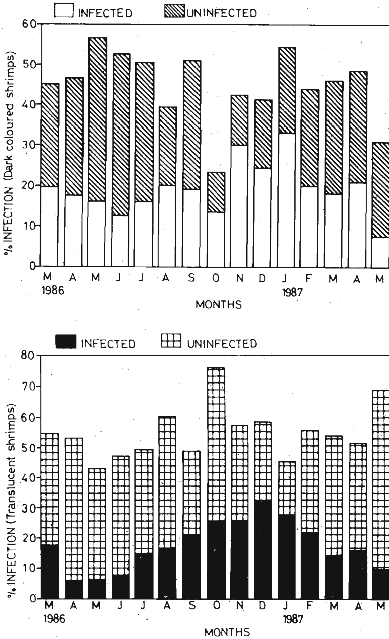
Figure 3 (a) : Comparison of the fluctuation in percentage of "Dark" coloured shrimps (The expression "Dark" has been used to demarcate shrimps with a gradation in colour from light brown to complete black) infected with the ecto-commensal Paracaridinicola . (b) : Comparison of the fluctuation in the percentage of translucent shrimps infected with Paracaridinicola .
