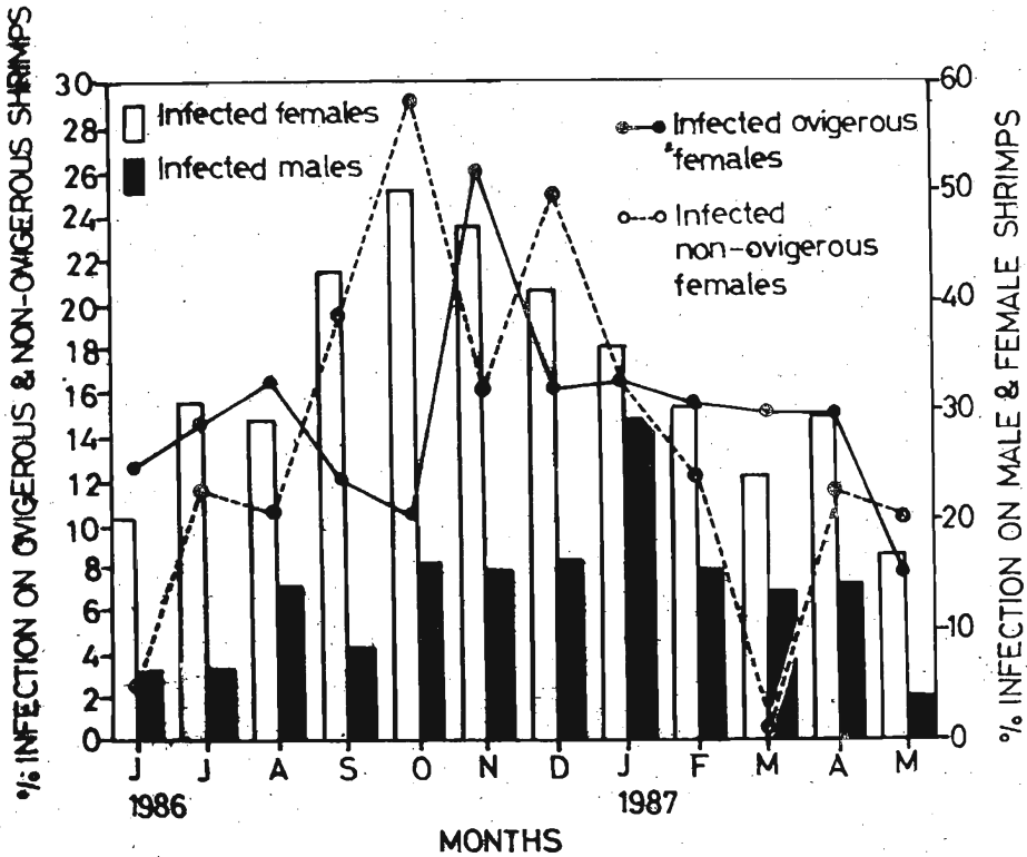
Figure 2 : Monthly fluctuation in the percentage of male and female shrimps and ovigerous and non-ovigerous females infected with Paracaridinicola platei .
