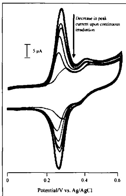
Figure 4.3: Cyclic voltammograms recorded during a 25 hour period of photo-oxidation of HT (0.6 mM) in 0.1 M acetate buffer (pH 4.0), at a scan rate of 50 mV s -1 .
