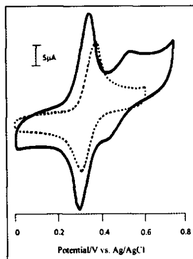
Figure 2: Cyclic voltammograms obtained on a glassy carbon electrode in 0.1 M acetate buffer (pH 4.0) containing (a) 0.1 mM HT (solid line), (b) 0.2 mM catechol (dashed line), at a scan rate of 50 \text{ mV s}^{-1} .
