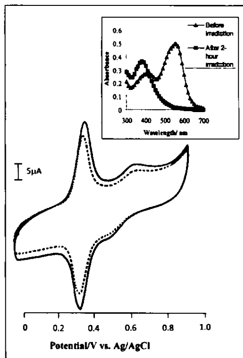
Figure 4.2: Cyclic voltammograms of HT in acetate buffer (pH 4.0) before the irradiation (solid line) and after two hours of irradiation (dashed line), at a scan rate of 50 \text{ mV s}^{-1} . The inset shows the corresponding absorption spectra as a function of time.
