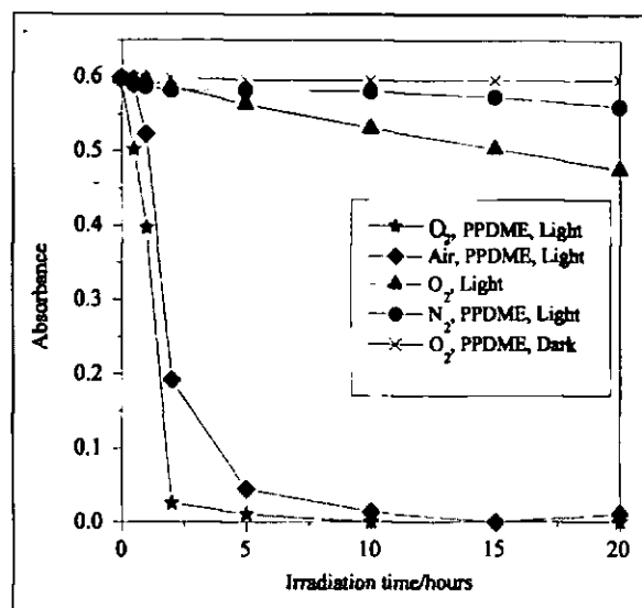
Figure 5: Change in absorbance, measured at 560 nm, for the disappearance of magenta colour of HT, upon irradiation under different conditions.
