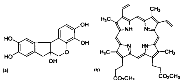
Figure 1: The chemical structure of hematoxylin (a) and protoporphyrin dimethylester (b).
