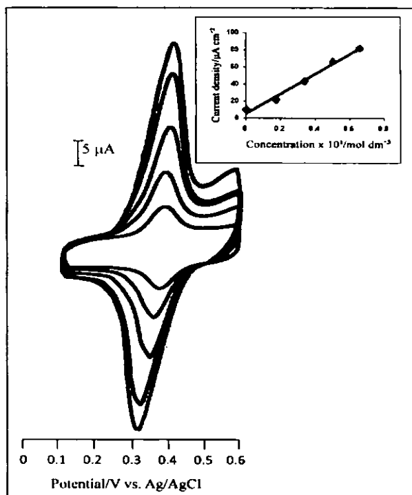
Figure 3: Cyclic voltammograms of HT, when its concentration is varied from 0.005 mM to 0.750 mM in the acetate buffer (pH 4.0) on a glassy carbon electrode at a scan rate of 50 \text{ mV s}^{-1} . The inset shows the plot of current density vs. concentration of HT.
