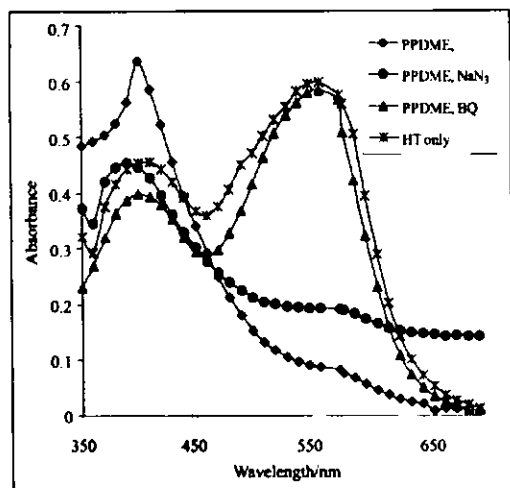
Figure 6: Spectral profiles showing the scavenging effect of BQ and \text{NaN}_3 on photobleaching of air-saturated solution of HT under 2 hour irradiation.
