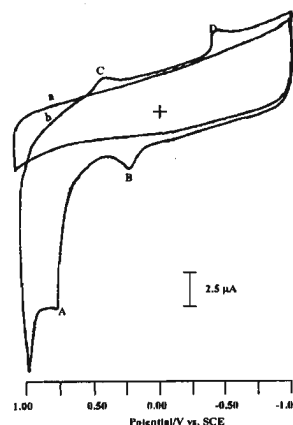
Figure 1: Cyclic voltammogram of Thiram in 0.1 M KCl at a scan rate of 50 \text{ mV s}^{-1} under \text{N}_2 saturated. (a) supporting electrolyte only (b) 1.0 \times 10^{-4} M Thiram.
