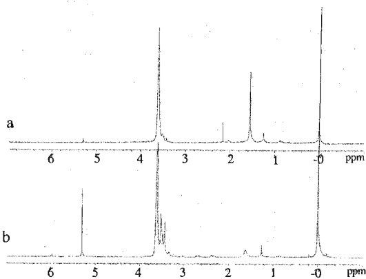
Figure 6: NMR spectra of (a) Commercial sample of Thiram (b) Residue of bean seed washings.
