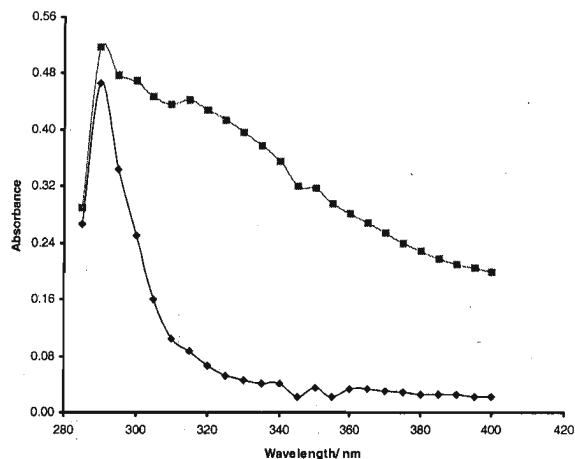
Figure 7: UV spectra of a 5.0 \times 10^{-5} M Thiram standard solution ( \blacklozenge ) and the residue of bean seed washings ( \blacksquare ).
