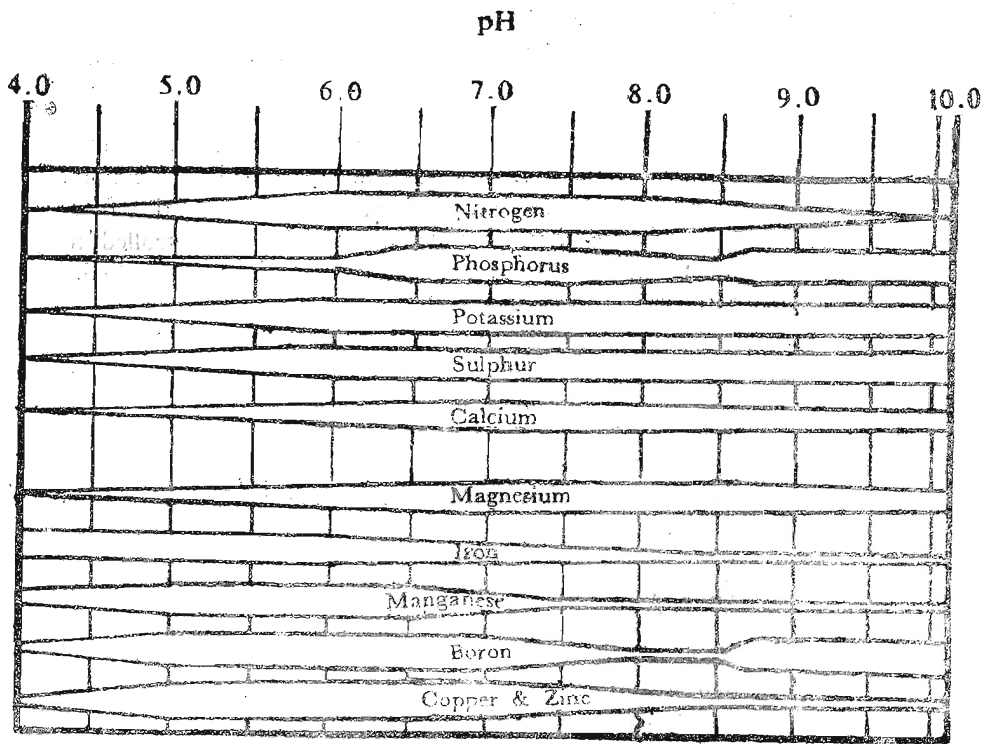
Figure 2.1 Diagrammatic representation of the availability of nutrients with change of pH (After Truog*)
