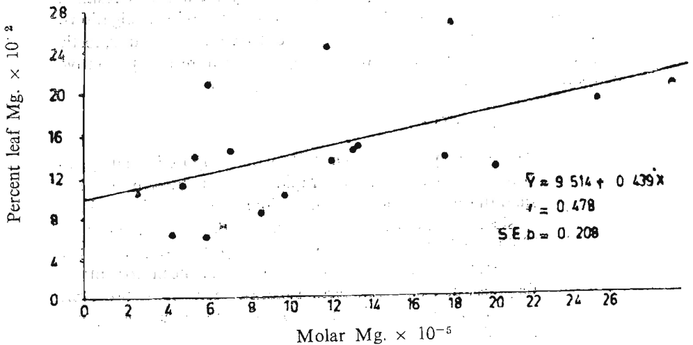
Figure 6.1 The relationship between leaf magnesium and the molar magnesium content of soils extracted with 0.01 molar calcium chloride solution. (After Nethsinghe et al *)
