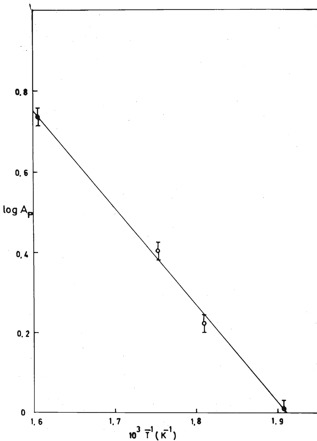
Figure 3. Plot of \log A_p (peak absorbance A_p in arbitrary units) vs T^{-1} .
