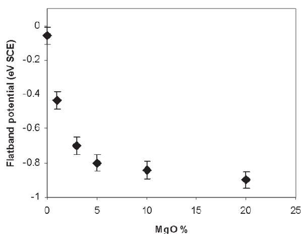
Fig. 2 Variation of flatband potential for SnO 2 with the change of % of MgO at pH 5.0.
