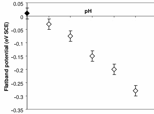
Fig. 1 Variation of flatband potential for \text{SnO}_2 as a function of solution pH.
