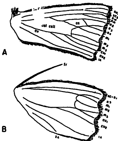
Figure 5. Wing venation of noctuid moth found on P. ostreatus . A. fore wing, B. hind wing, fr- frenulum.
