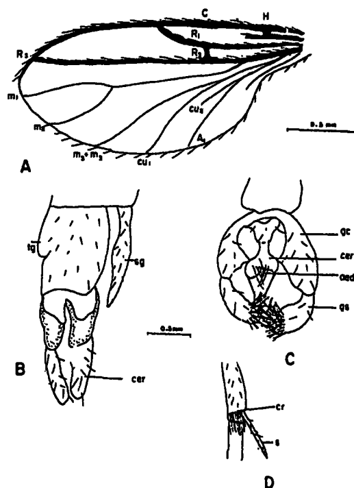
Figure 3. Morphological structures of taxonomic importance of Bradysia paupera adult. A. Fore wing, B. Female genitalia C. Male genitalia D. Pro tibia of male showing characteristic arrangement of bristles ade-adeagus, cer-cercus, cr-crest of bristles, gc-gonocoxite, gs-gonostyle, sp-spur, s9-9th abdominal sternum, t9-ninth abdominal tergum.
