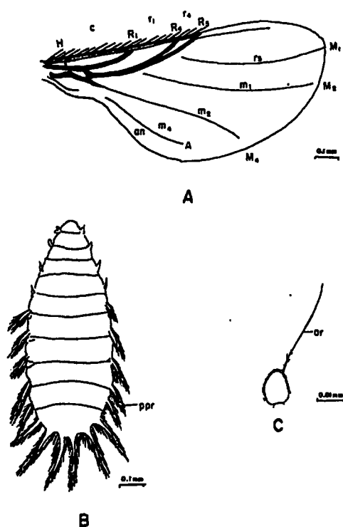
Figure 2. Features of taxonomic importance of Megaselia halterata (Wood). A. wing venation B. larva C. antenna. ar. arista, ppr. plumose projection (six in posterior portion)
