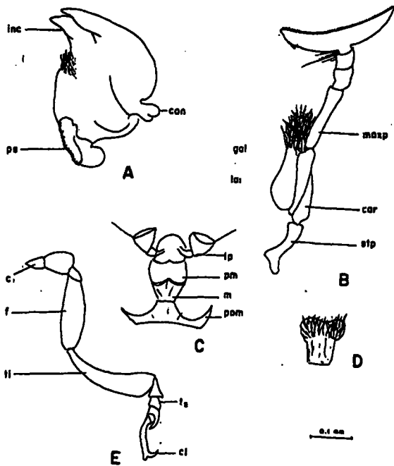
Figure 4. Morphological structures of taxonomic importance of Triples sp. A. Mandible (left), B. Maxilla (left), C. Labium, D. Labrum, E. leg, cl- claw, car- cardo, c- coxa, con- condyle, f- femur, gal- galea, inc- incisor, la- lacinia, lp- labial palp, m- mentum, maxp- maxillary palp, pm- prementum, ps- prosthema, p m- postmentum, stp- stipe, ti- tibia, t2- second taxsomere
